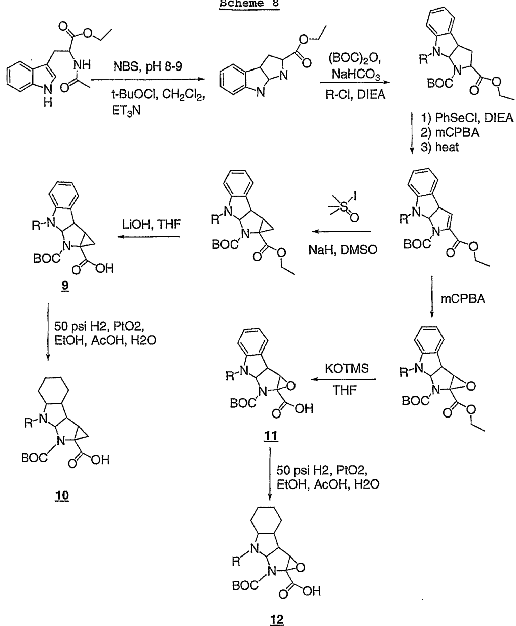
Scheme 8
