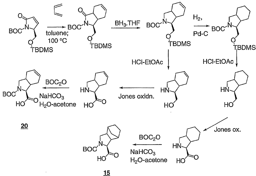
Scheme 14
