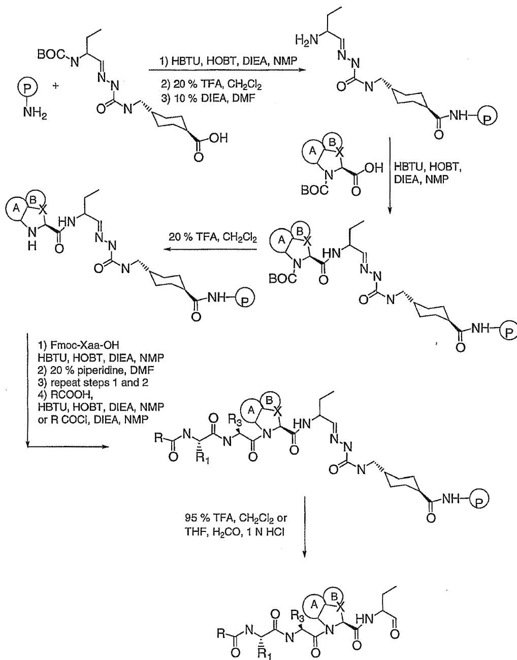
Scheme 16
