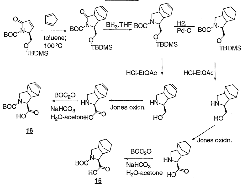
Scheme 10
