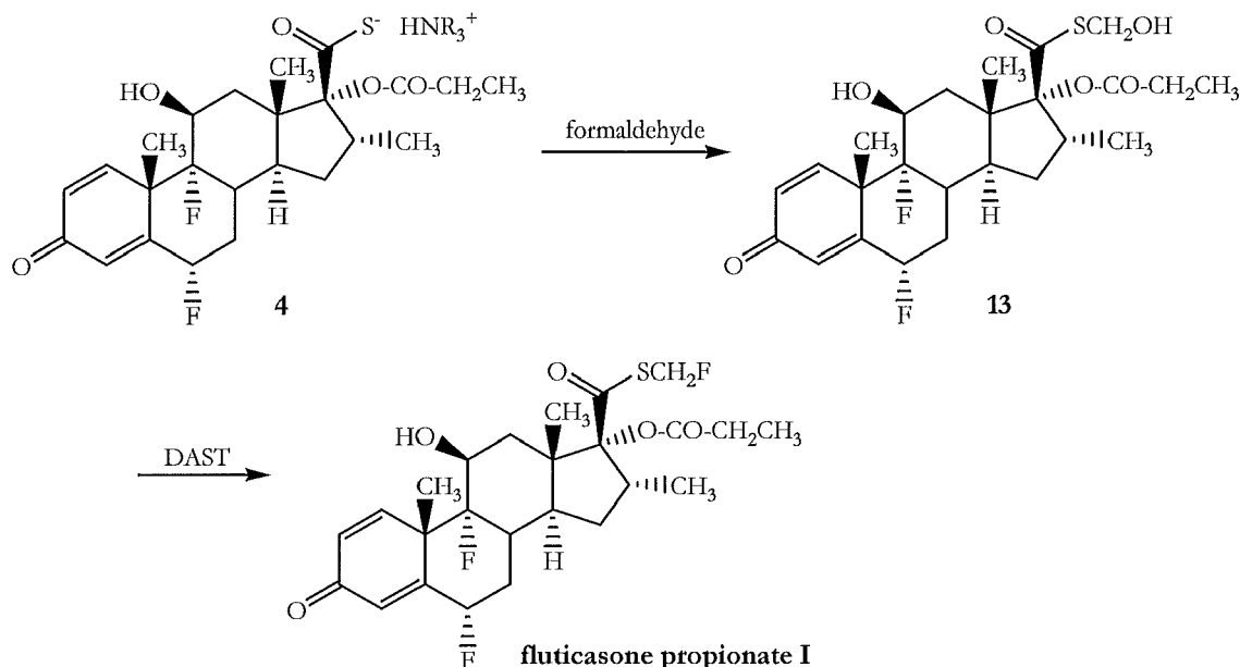
Scheme 5
