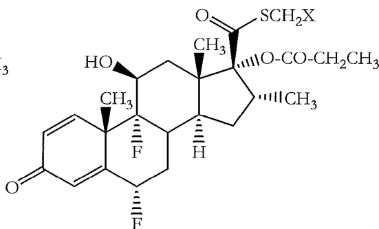
compound II
