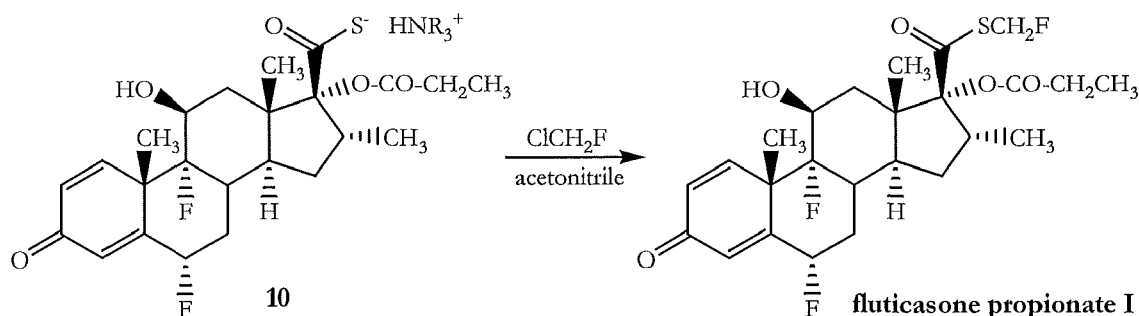
Scheme 4
