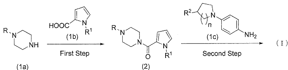
Reaction Scheme 1
