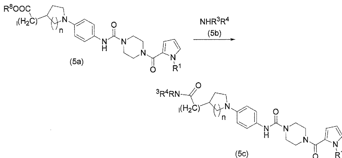
Reaction Scheme 5
