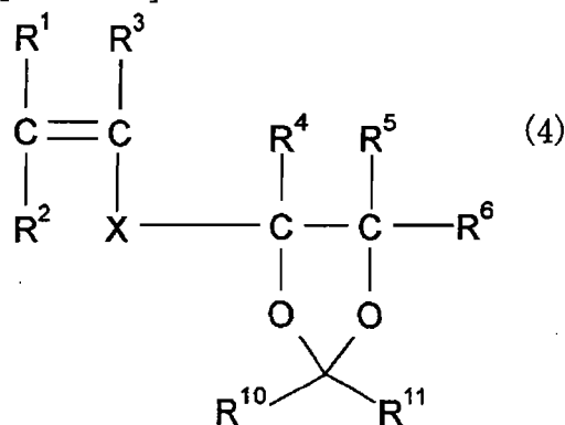
[Chem. 13]
