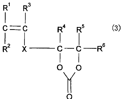
[Chem. 12]
