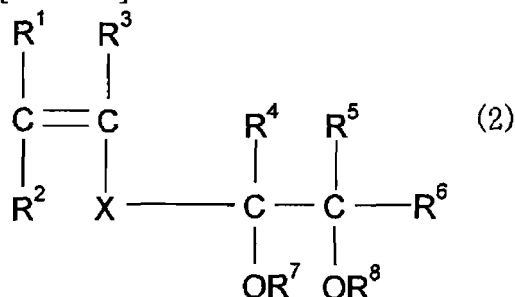
[Chem. 7]
