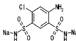
Compound No. 17
