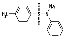
Compound No. 10
