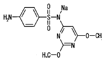
Compound No. 15
