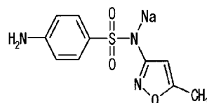
Compound No. 14
