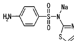
Compound No. 12
