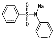
Compound No. 9
