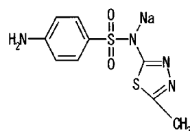
Compound No. 13
