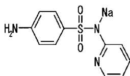
Compound No. 11
