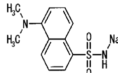
Compound No. 19
