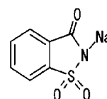
Compound No. 16
