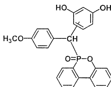
[Chemical formula 41]
