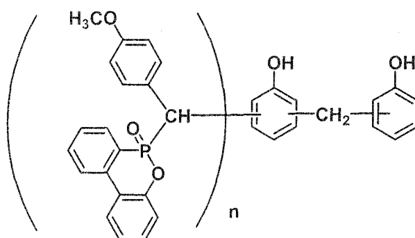
[Chemical formula 40]
