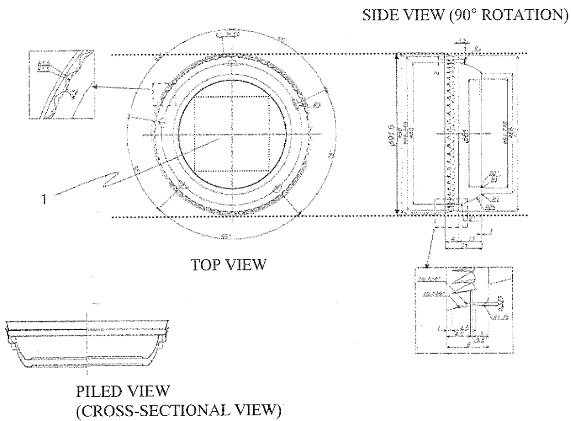
FIG. 1 VACUUM-FORMED ARTICLE (CUP-SHAPED)
