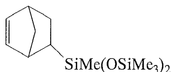
Monomer C
