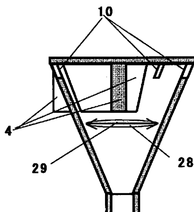
CROSS-SECTIONAL VIEW ALONG B-B
