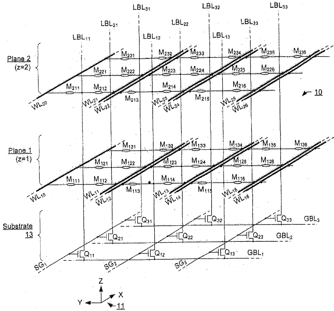
Single-Sided Word line Structure
