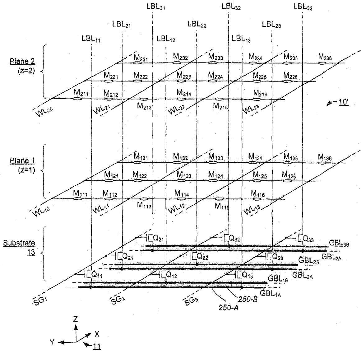
Double-Global-Bit-line Structure
