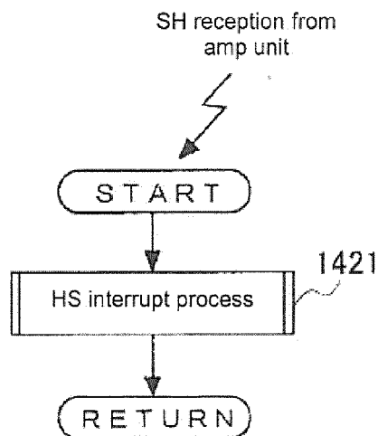
Fig. 14C HS reception interrupt processes
