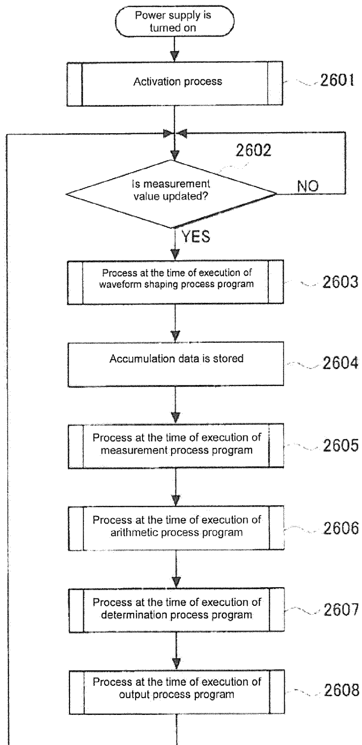
General flowchart showing processes of extension unit
