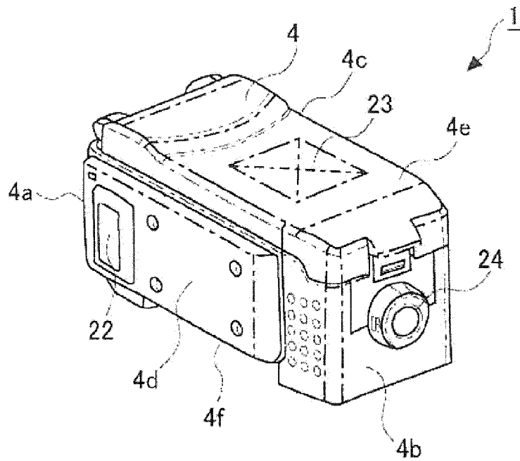
Fig. 6B Perspective view taken obliquely from behind
