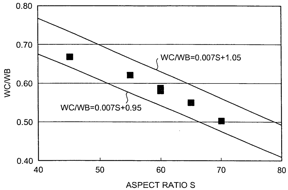
RELATIONSHIP BETWEEN WC/WB AND ASPECT RATIO S
