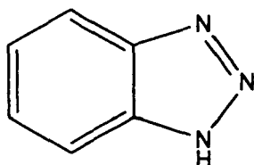
[Chem. 47]
