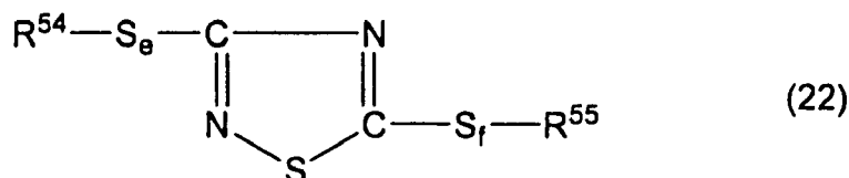
[Chem. 29]
