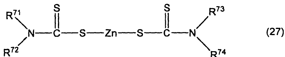
[Chem. 33]
