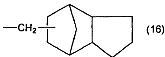
[Chem. 24]
