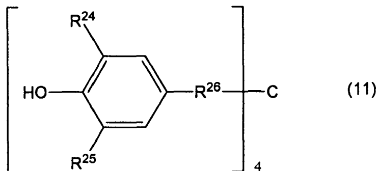
[Chem. 10]
