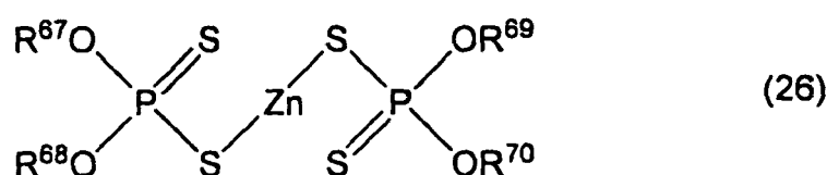
[Chem. 32]
