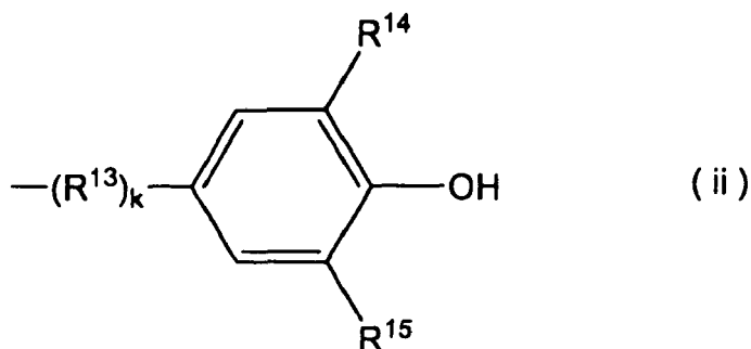
[Chem. 8]
