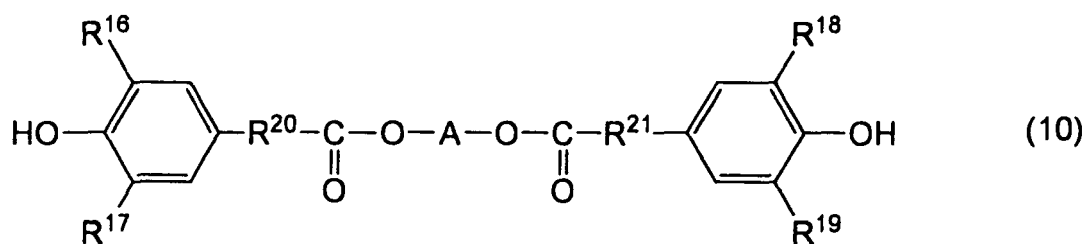
[Chem. 9]
