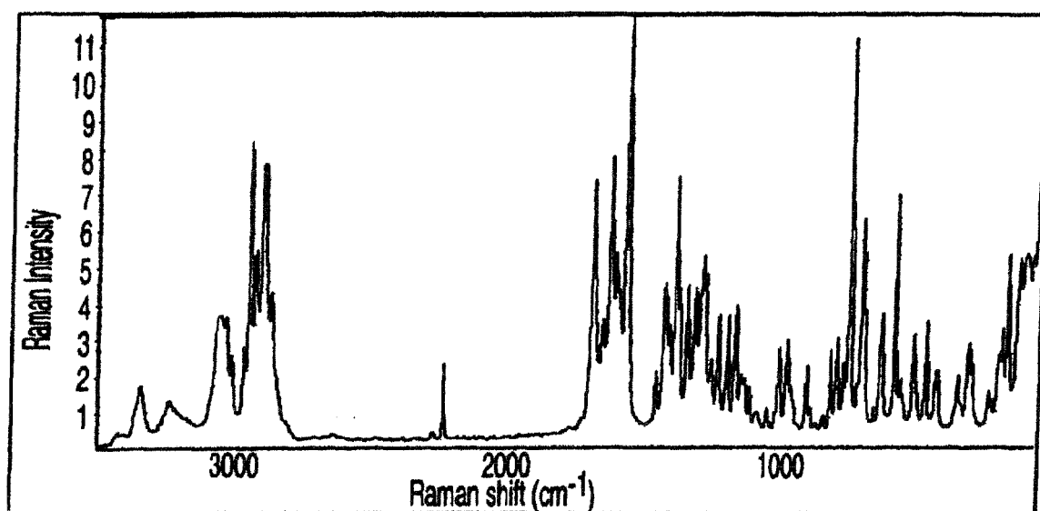
RAMAN SPECTRUM OF FORM D
