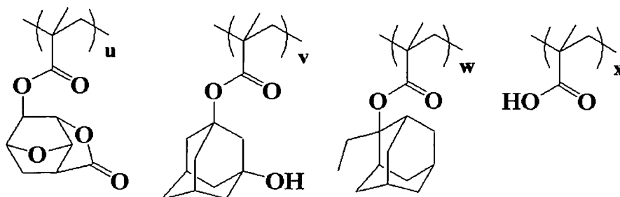
ArF monolayer resist polymer 1 ( u=0.45, v=0.20, w=0.30, x=0.05 Mw7,800)
