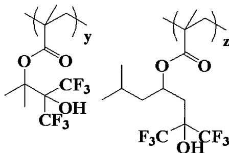
Water-shedding polymer 1 ( y=0.45, z=0.55 M_w 8,800 )
