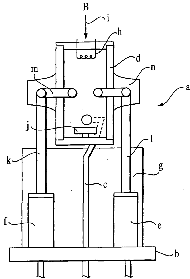
FIG. 1 PRIOR ART
