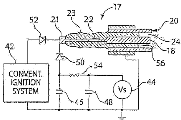
Fig. 2 (Prior Art)
