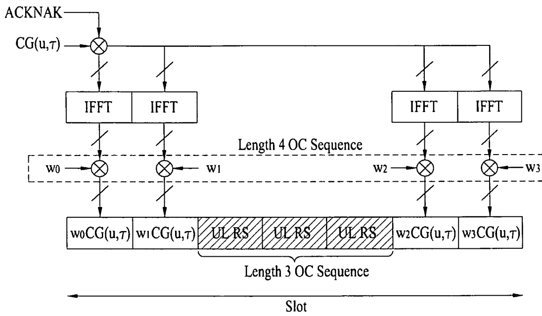
PUCCH format 1a and 1b structures (Normal CP)
