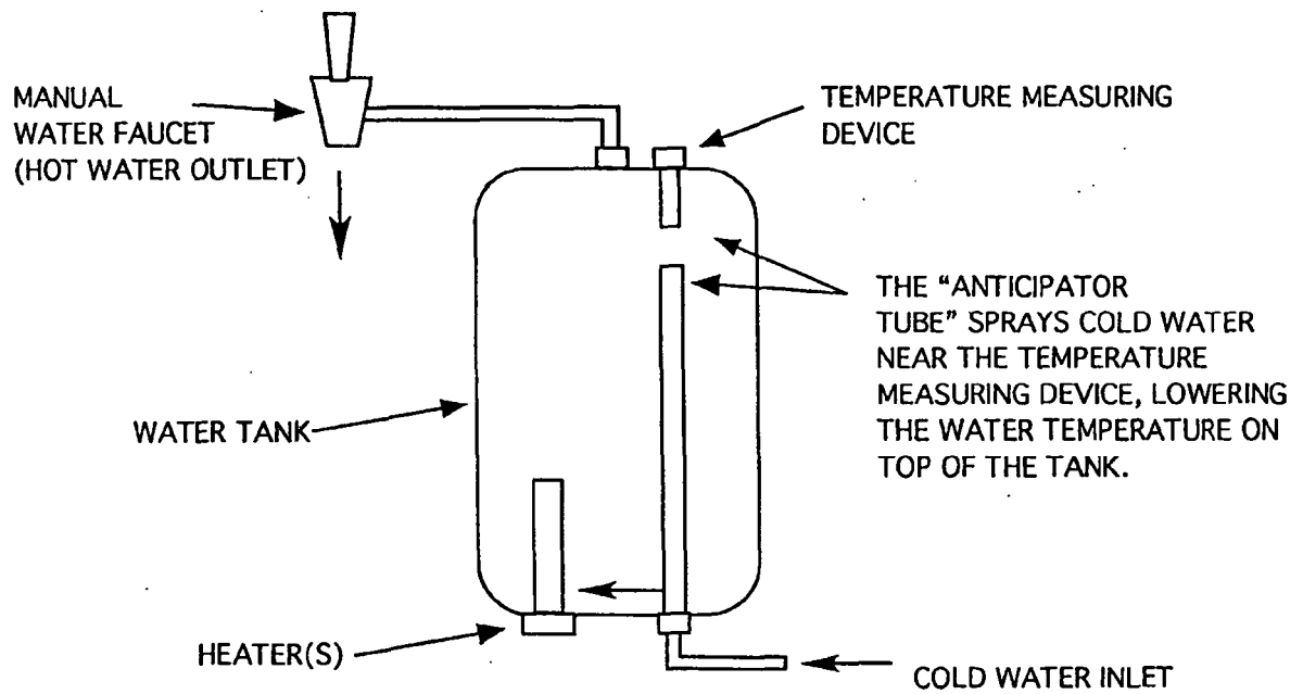
FIGURE 1 - TYPICAL PRIOR ART WATER HEATING SYSTEM
