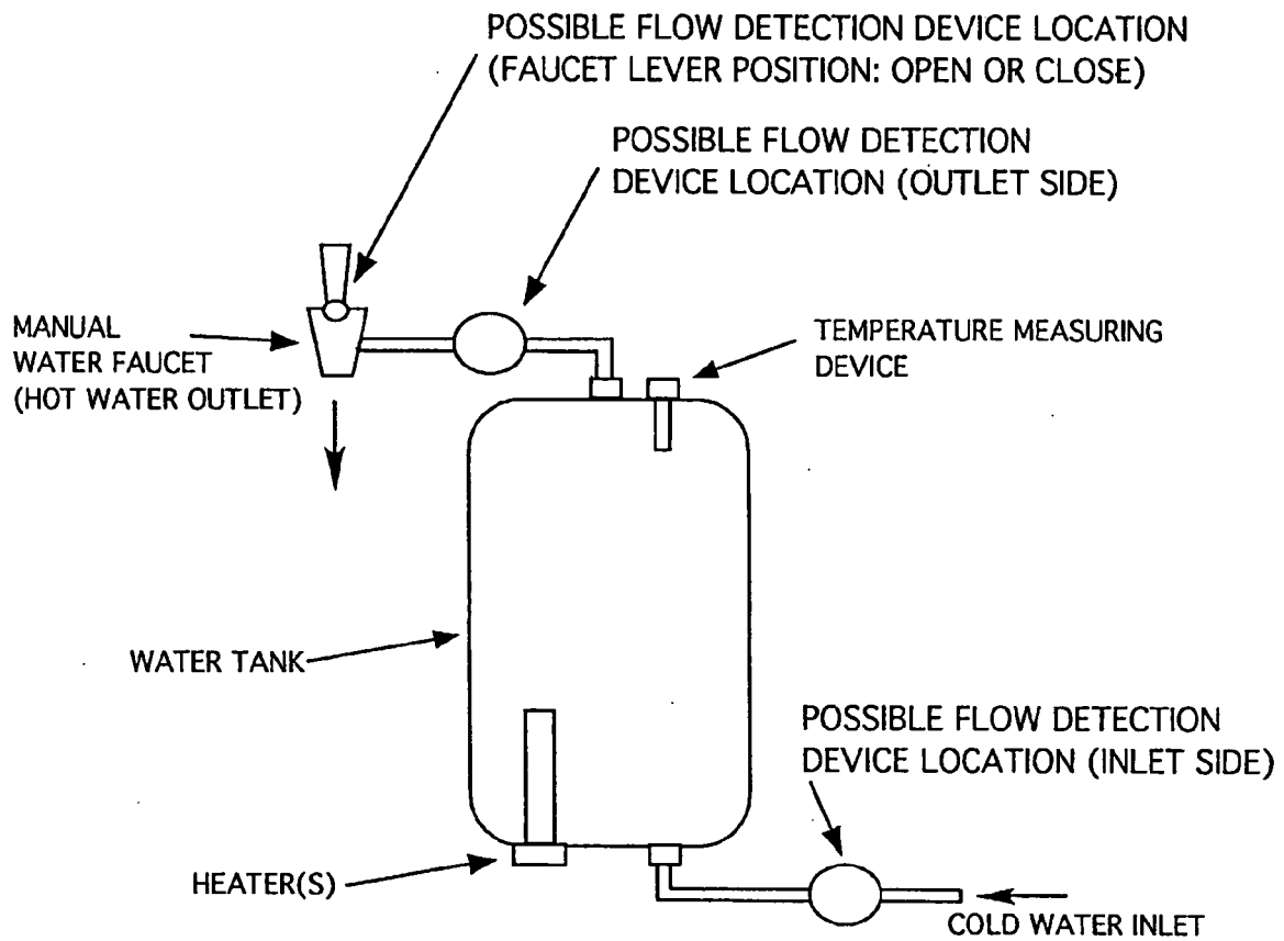
FIGURE 2 - IMPROVED WATER HEATING SYSTEM
