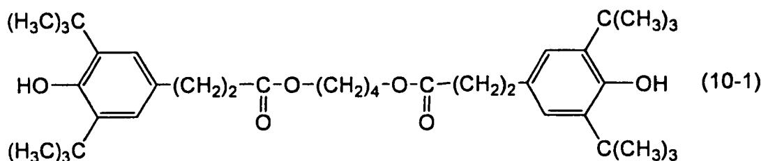
[Chem. 12]
