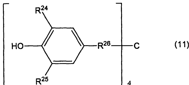
[Chem. 10]
