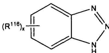
[Chem. 48]
