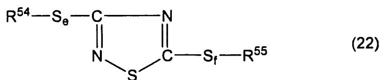
[Chem. 28]
