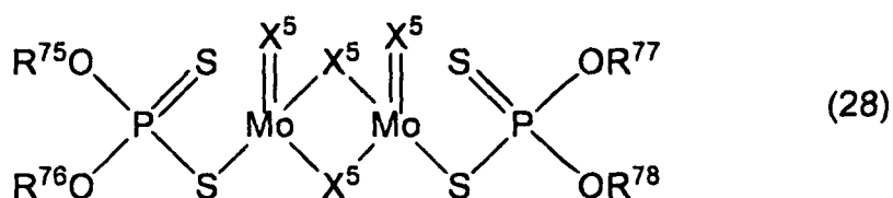
[Chem. 34]
