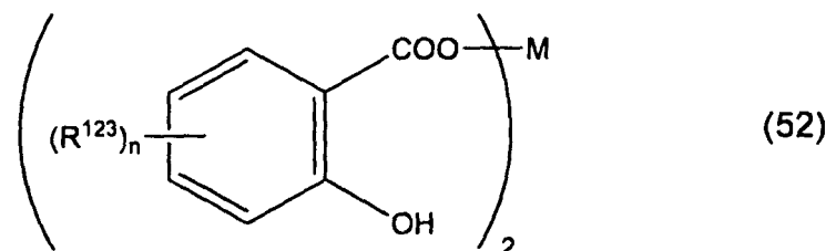
[Chem. 52]
