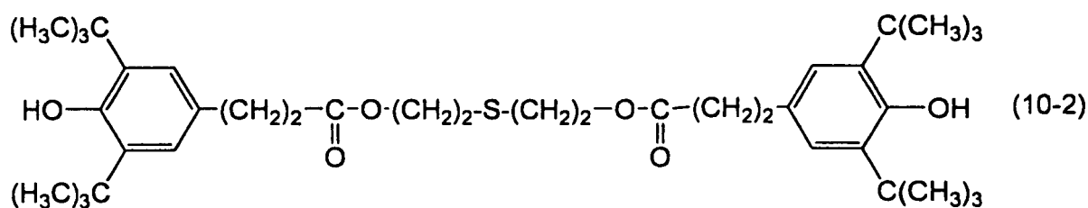
[Chem. 13]
