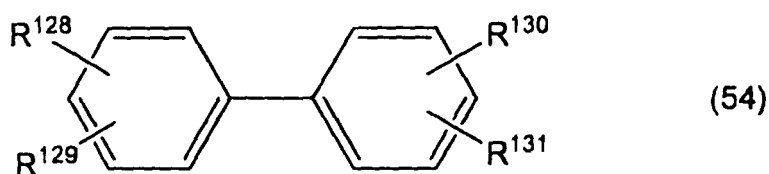
[Chem. 54]
