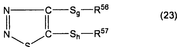
[Chem. 29]
