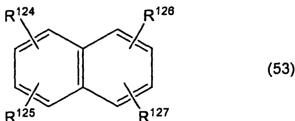
[Chem. 53]
