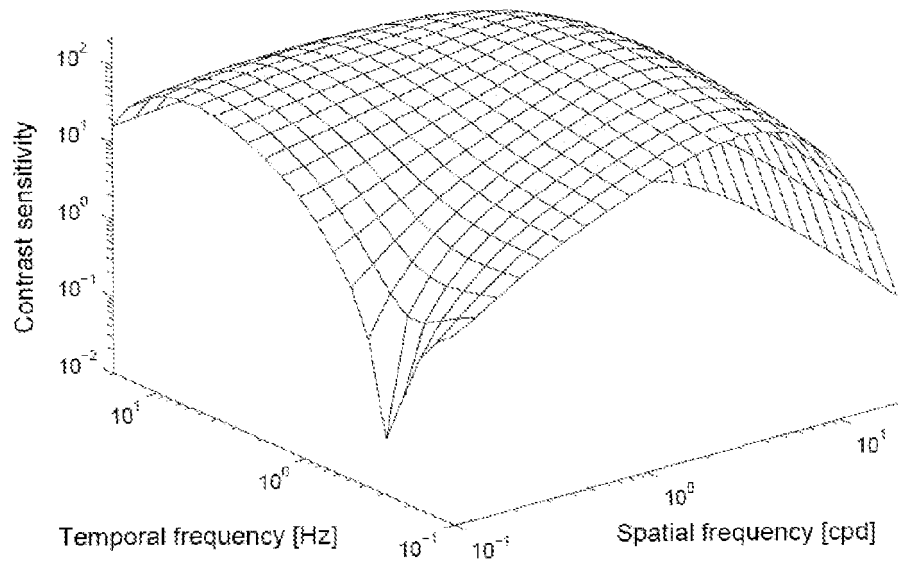
(a) Achromatic CSF
