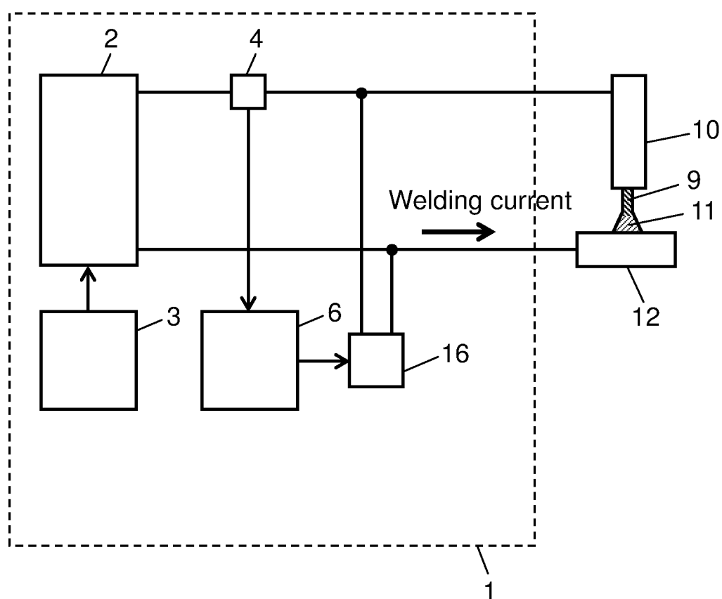
FIG. 9 PRIOR ART
