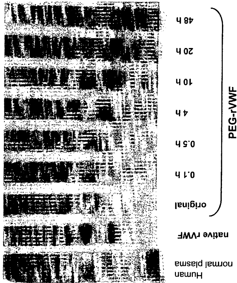
Figure 2 : Influence of pH- and amine-dependent PEG release on the multimeric structure of PEGylated rVWF
