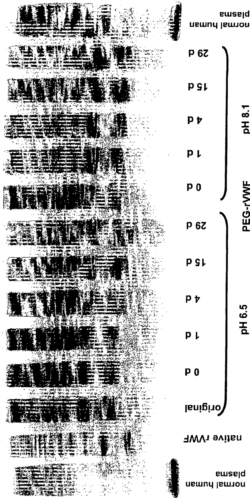
Figure 1: Influence of pH-dependent PEG release on the multimeric structure of PEGylated rVWF
