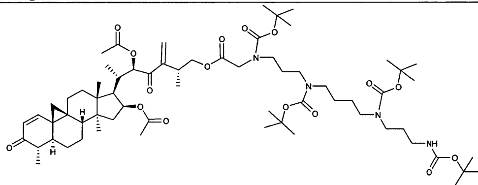
Compound 70
