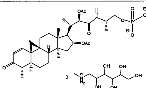
Compound 73
