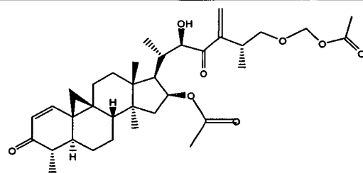
Compound 68
