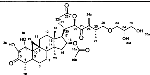
28 Compound 67
