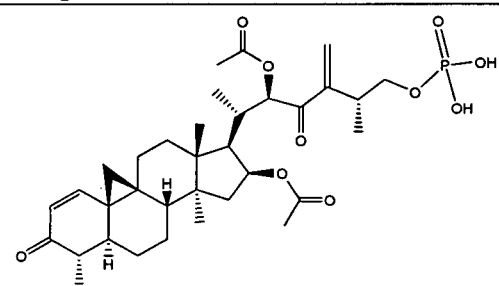
Compound 72
