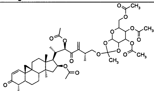
Compound 69
