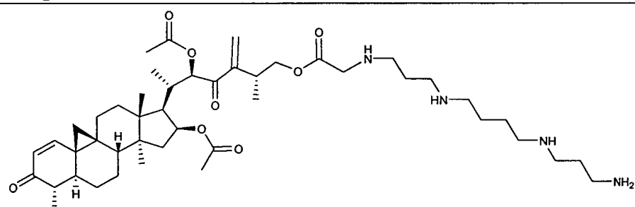
Compound 71
