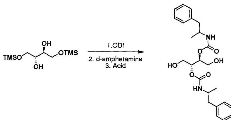
Scheme 12
