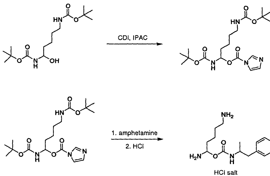
Scheme 9
