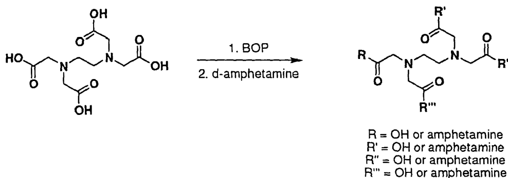
Scheme 18
