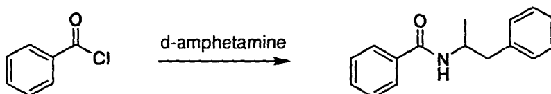
Scheme 14
