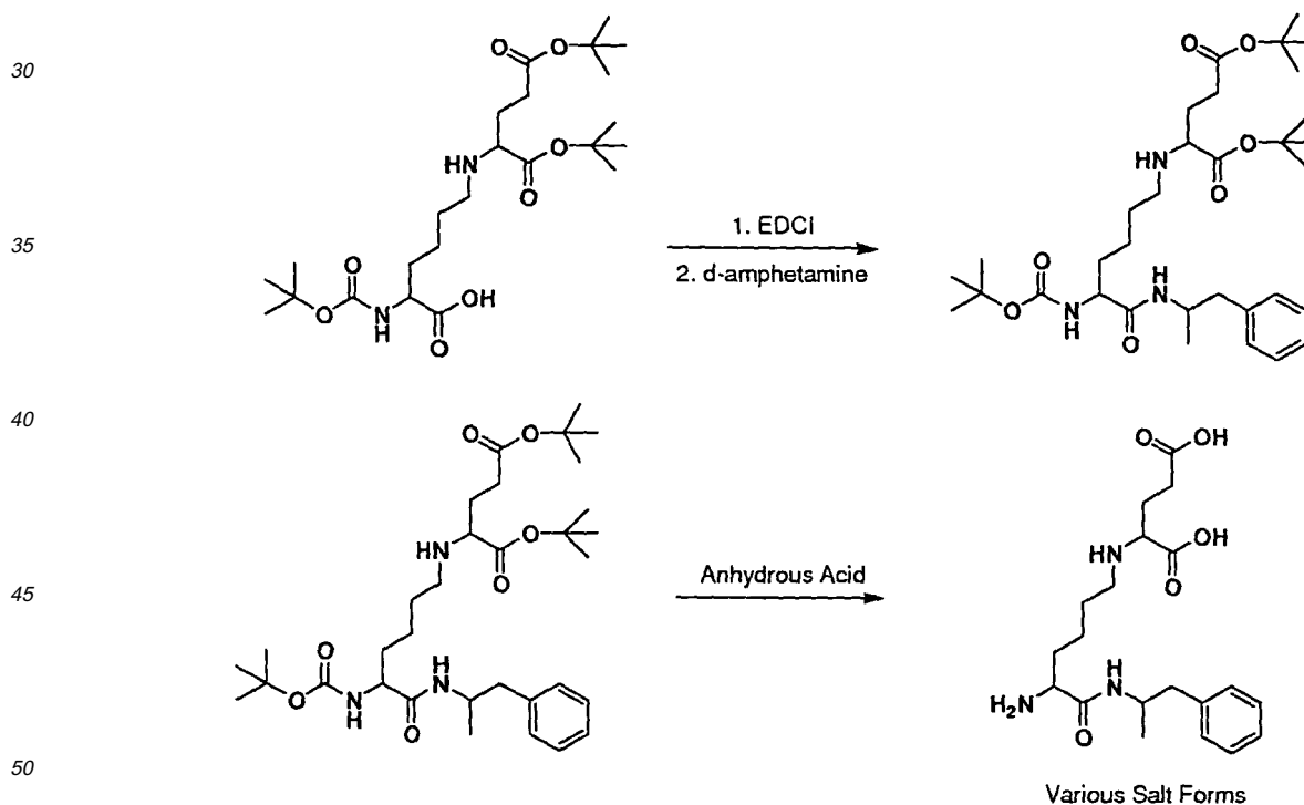
Scheme 5
