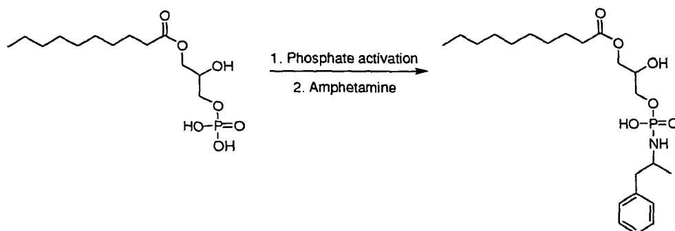
Scheme 13
