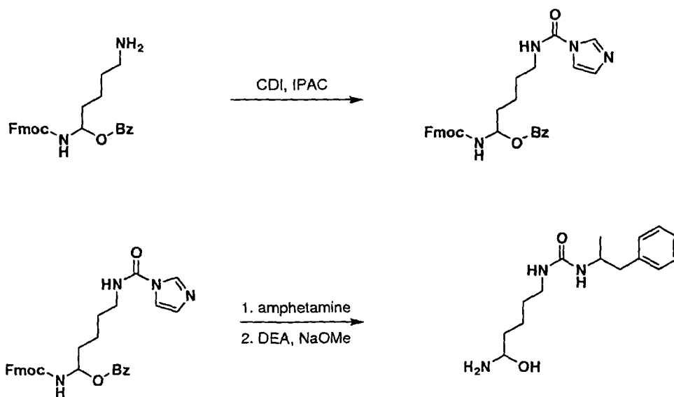
Scheme 10
