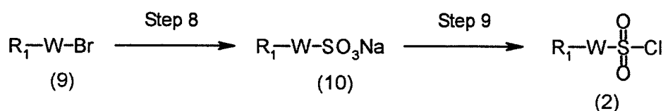
Scheme 4a
