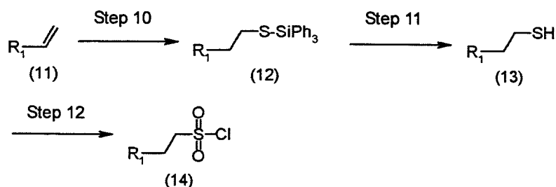
Scheme 4b
