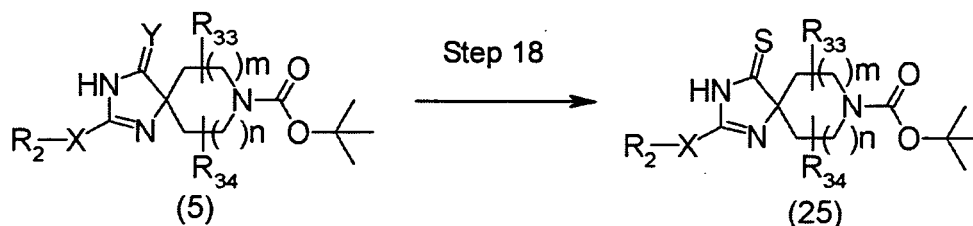
Scheme 10
