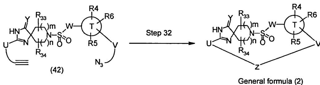
Scheme 23
