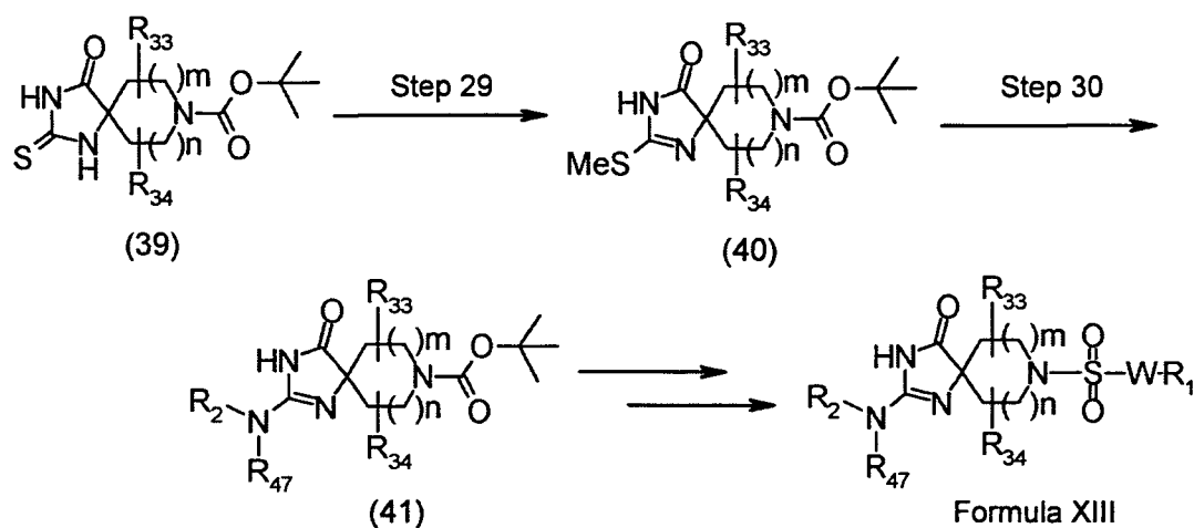
Scheme 20
