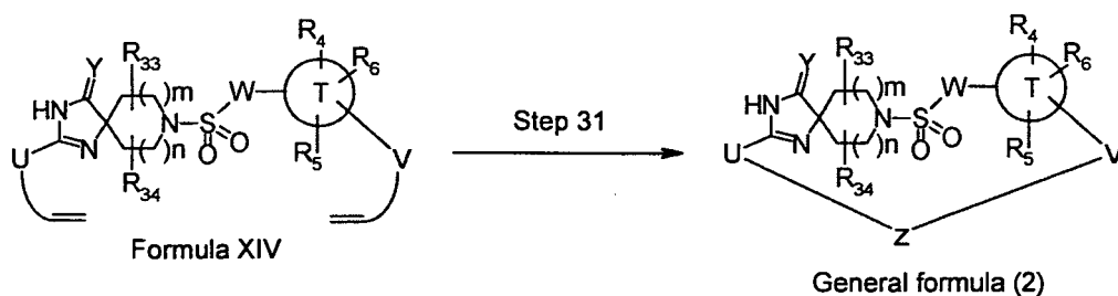
Scheme 21
