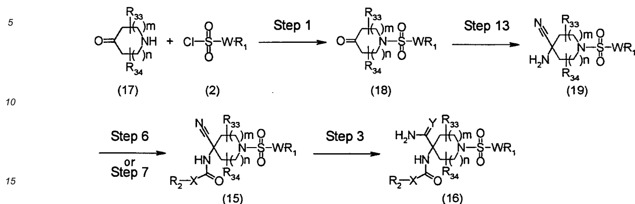
Scheme 6
