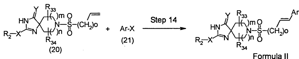
Scheme 7 (Method C)
