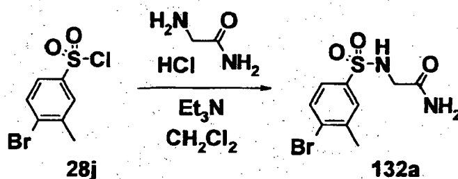
(Reaction 132-2)
