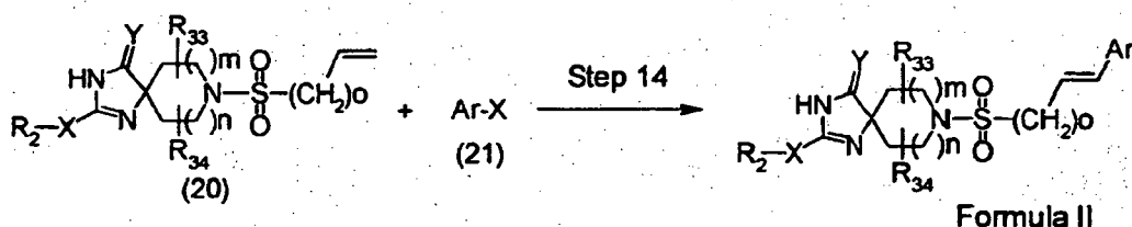
Scheme 7 (Method C)
