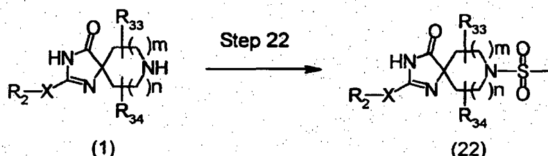
Scheme 13
