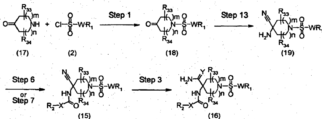
Scheme 6
