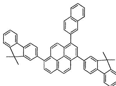
BD7 E^T=2\text{eV} Affinity=2.8eV Main peak wavelength 436nm
