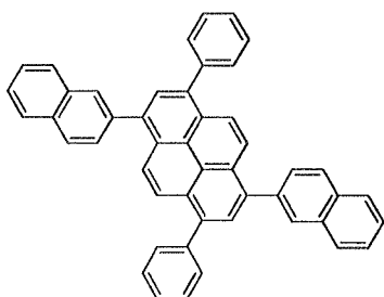
BD6 E^T=1.94\text{eV} Affinity=2.9eV Main peak wavelength 434nm
