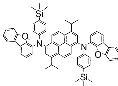
BD4 E^T=1.94\text{eV} Affinity=2.8eV Main peak wavelength 452nm
