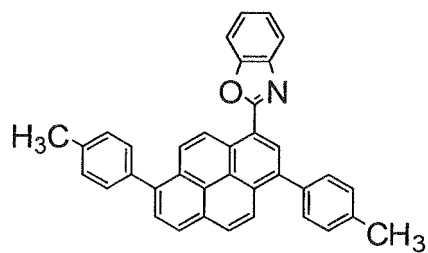
BD5 E^T=1.95\text{eV} Affinity=2.85eV Main peak wavelength 444nm
