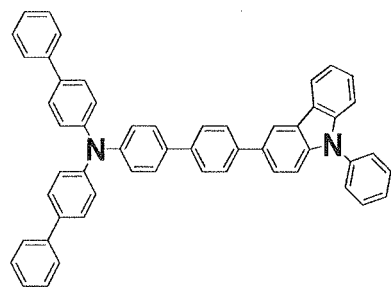
HT3 E^T=2.6\text{eV}
