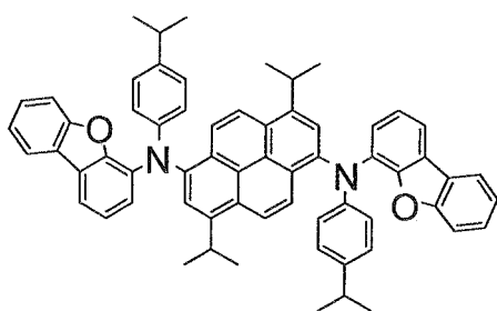
BD3 E^T=1.94\text{eV} Affinity=2.7eV Main peak wavelength 457nm
