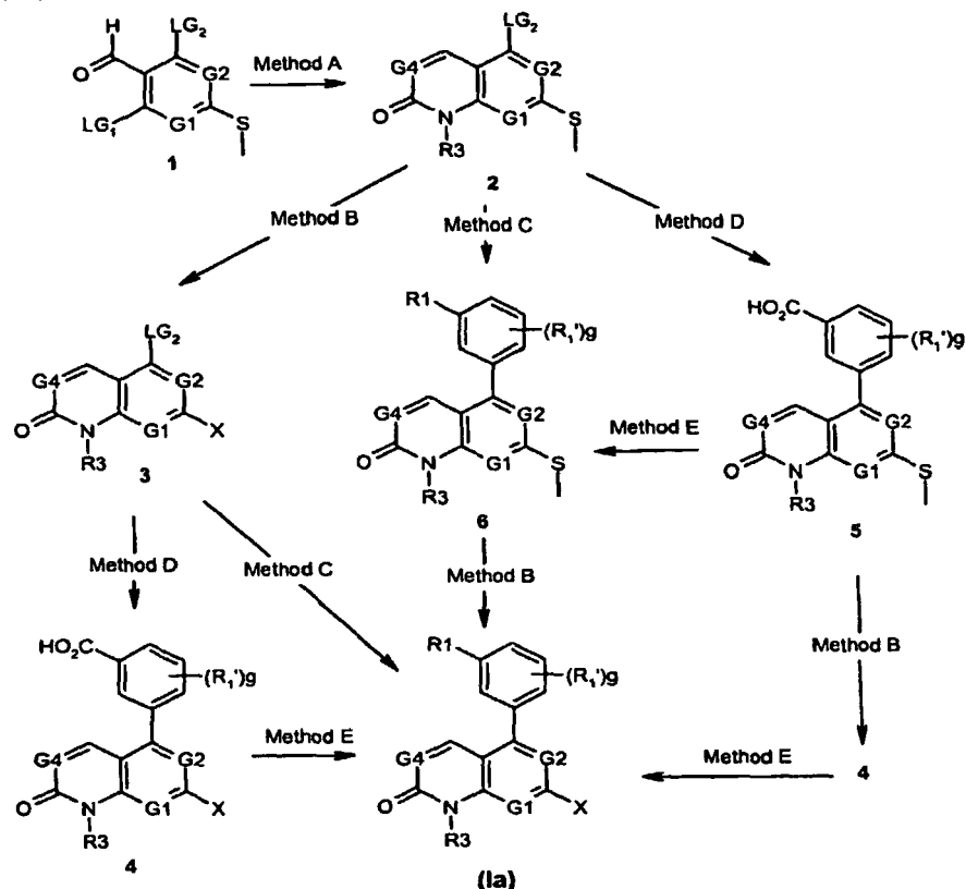
Scheme 1
