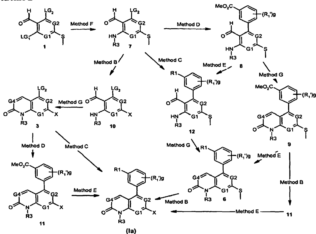
Scheme 2
