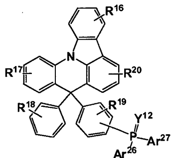
[Chemical Formula 7]
