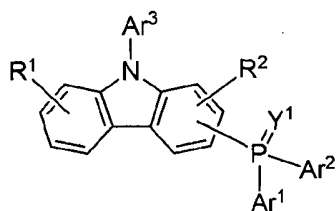
[Chemical Formula 1]
