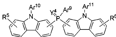
[Chemical Formula 3]
