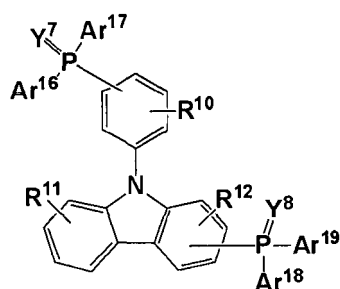
[Chemical Formula 5]
