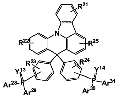
[Chemical Formula 8]
