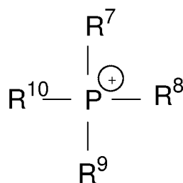
Phosphonium
