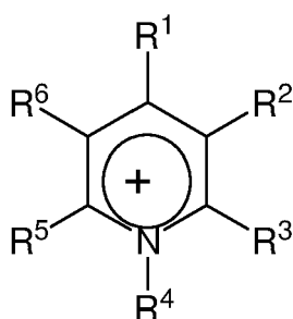
Pyridinium
