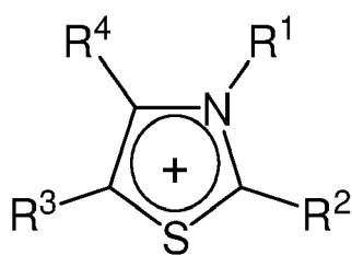
Thiazolium
