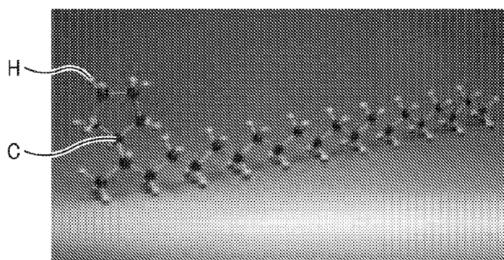
EXAMPLE OF CYCLOPARAFFIN
