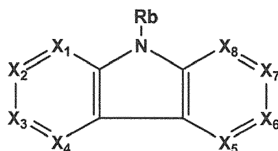
Formula (a)
