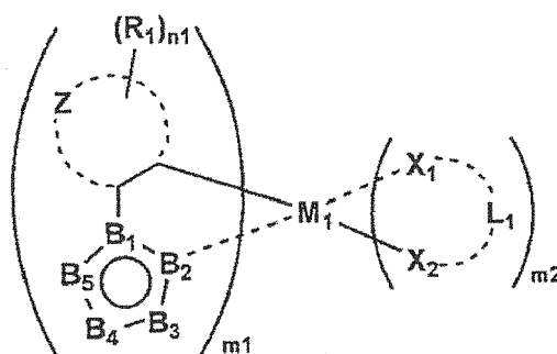
Formula (B)
