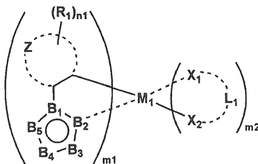
Formula (B)
