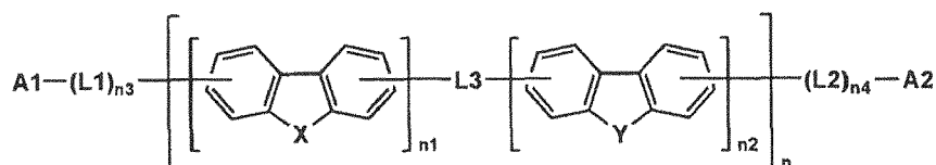
Formula (A)
