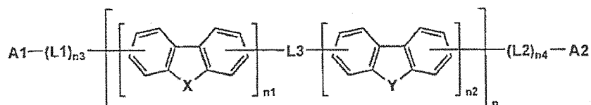
Formula (A)
