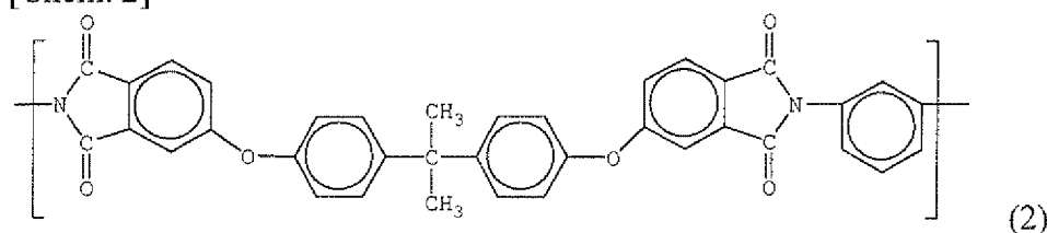
[Chem. 2]
