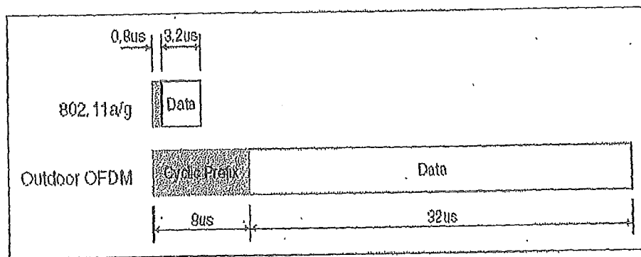
Figure 9 OFDM symbol dimensions
