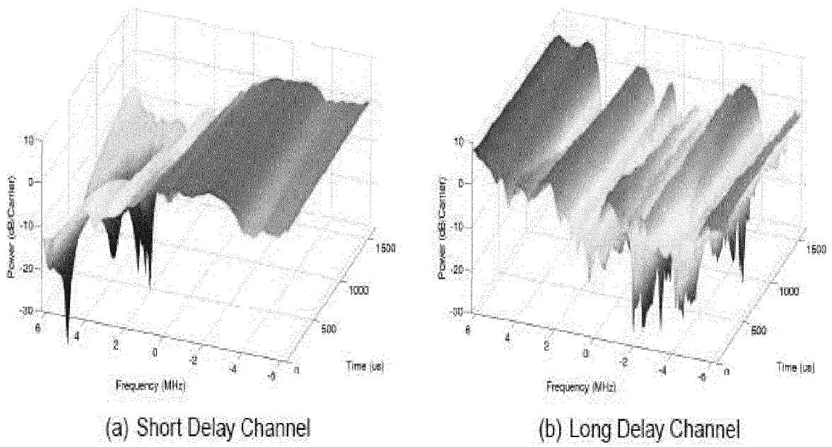
Figure 7: Mobile Channel Captures at 60 mph
