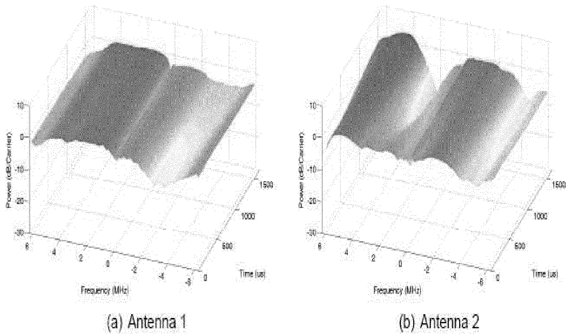
Figure 8: Radio Channel to Two Antennas 1m Apart
