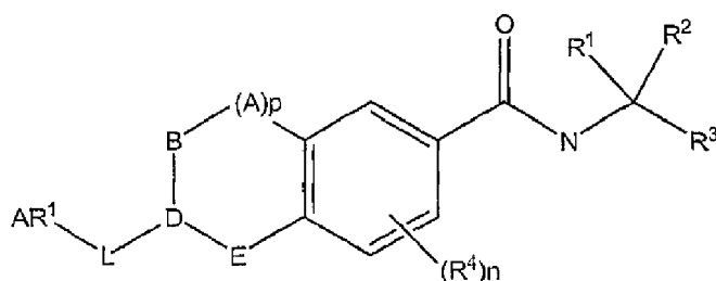
Formula 1
