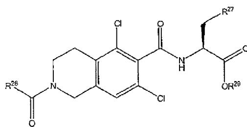
Formula II'
