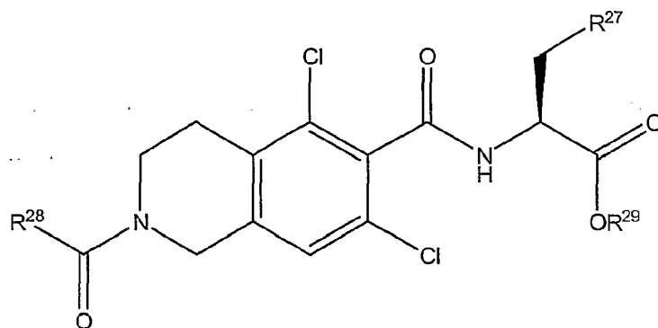
Formula II'
