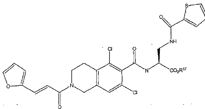
Formula IIA
