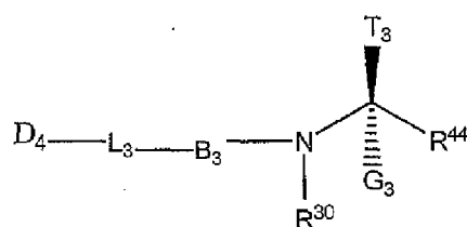
Formula VI
