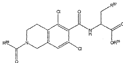
Formula II
