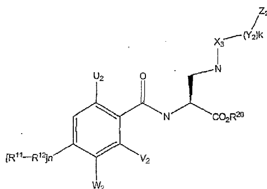
Formula III'
