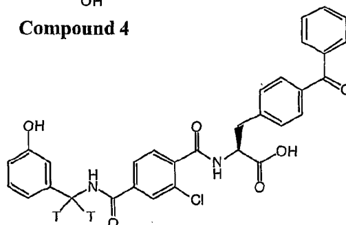
Compound 5
