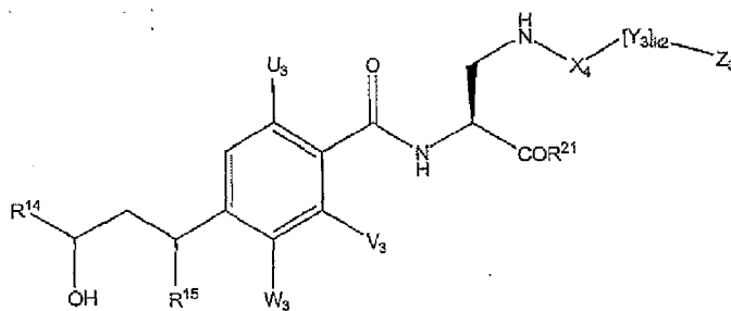
Formula V
