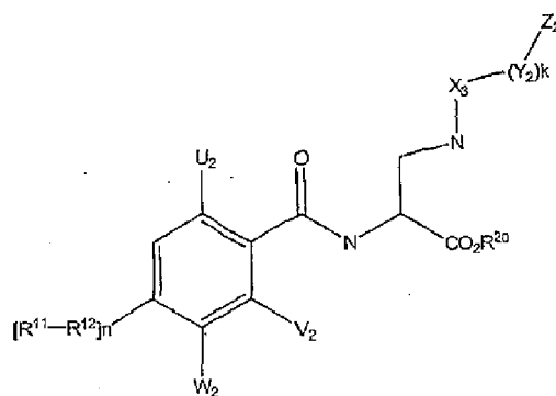
Formula IV
