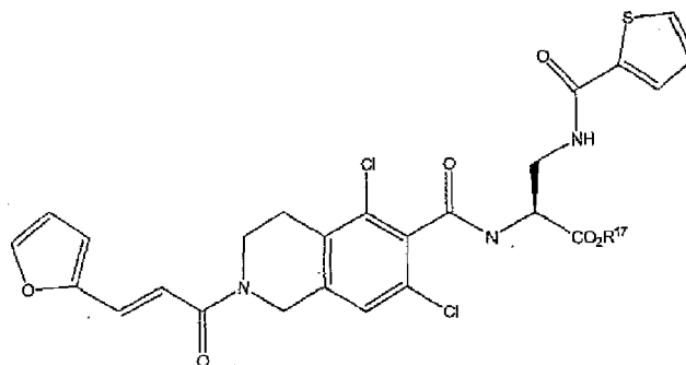
Formula IIA
