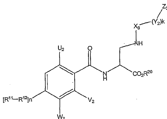
Formula IV
