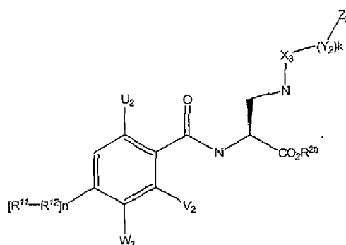
Formula IV'
