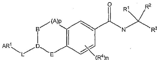
Formula 1
