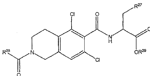
Formula II
