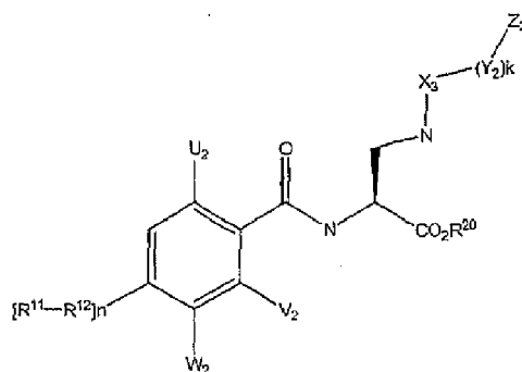
Formula IV'
