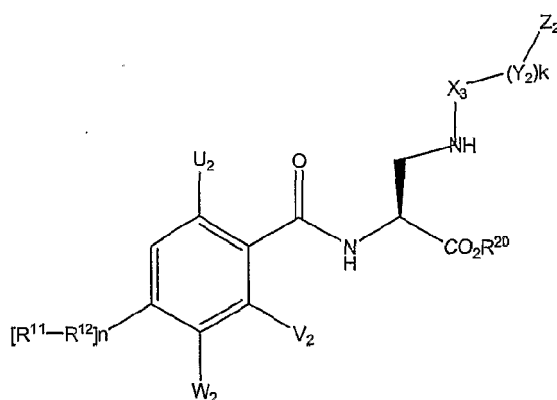
Formula IV'
