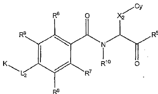
Formula III
