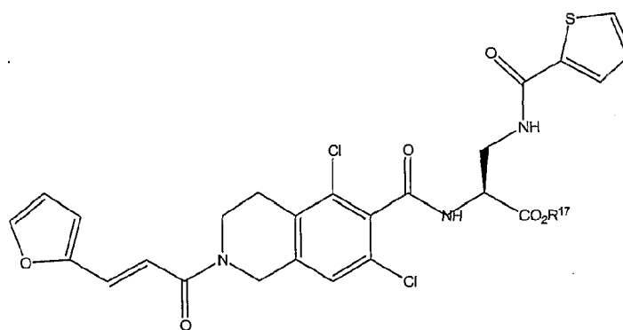
Formula IIA
