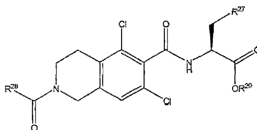
50 Formula II'
