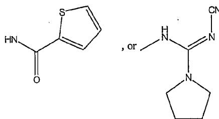
Formula II
