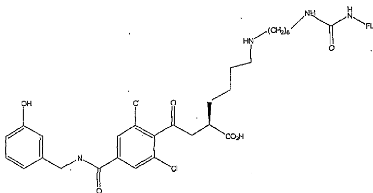
Formula VII
