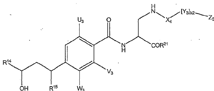
Formula V
