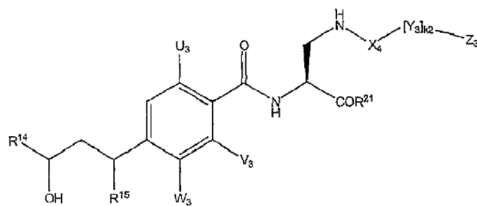
Formula V
