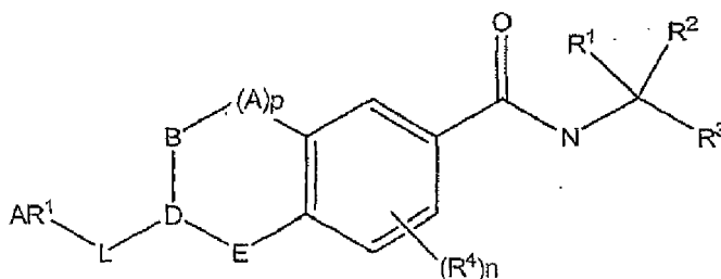
Formula 1
