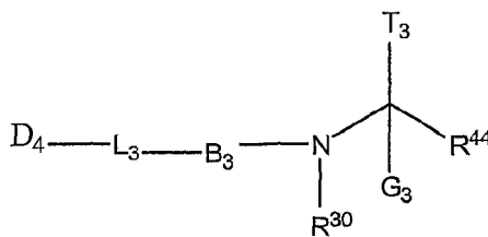
Formula VI
