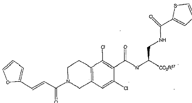
Formula IIA
