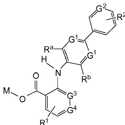
Formula (I-a)
