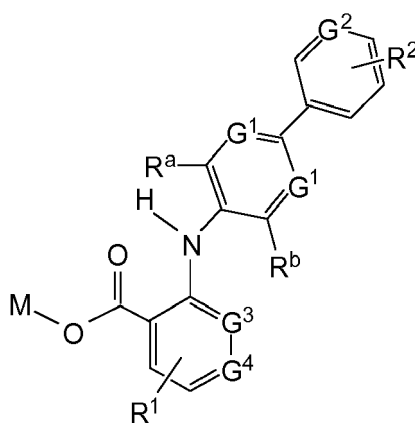
Formula (I-a)
