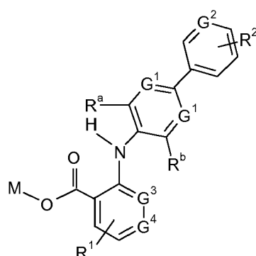
Formula (I-a)
