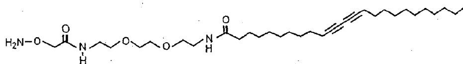
4 Photopolymerizable hydroxylamino derivative
