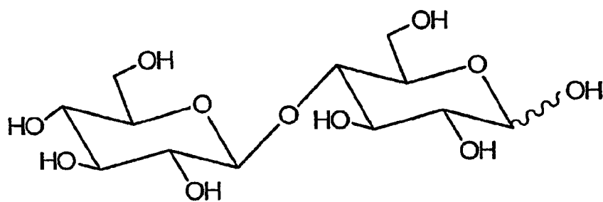
FIG. 5 Structure of Cellobiose
