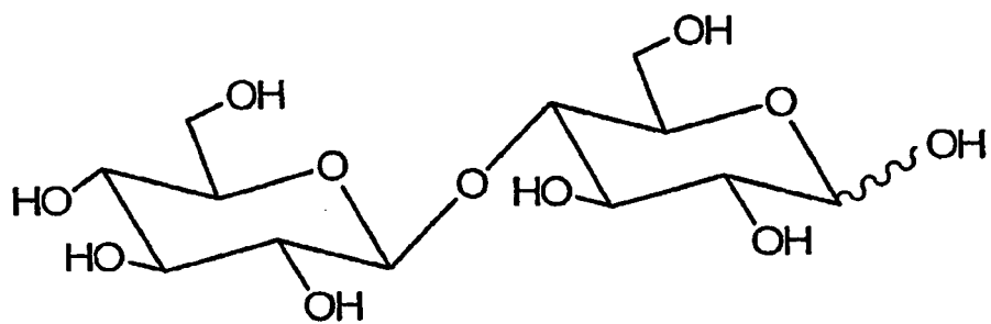
FIG. 5 Structure of Cellobiose
