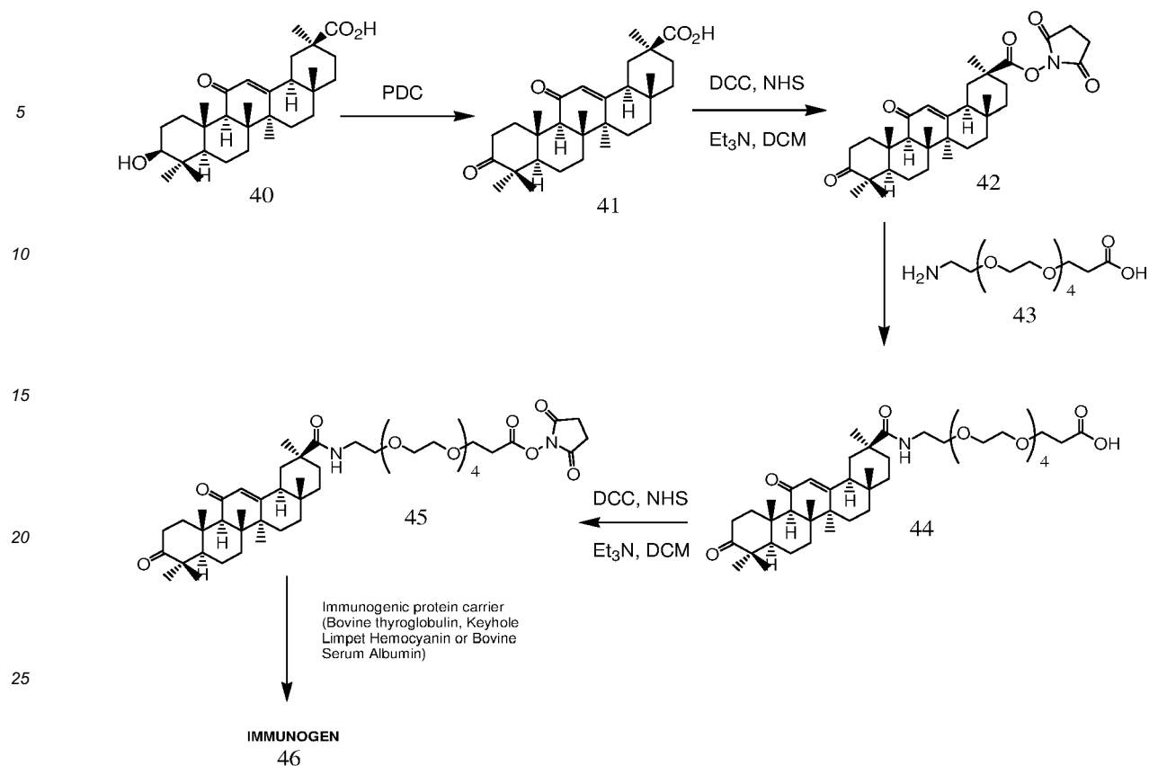
Scheme 6
