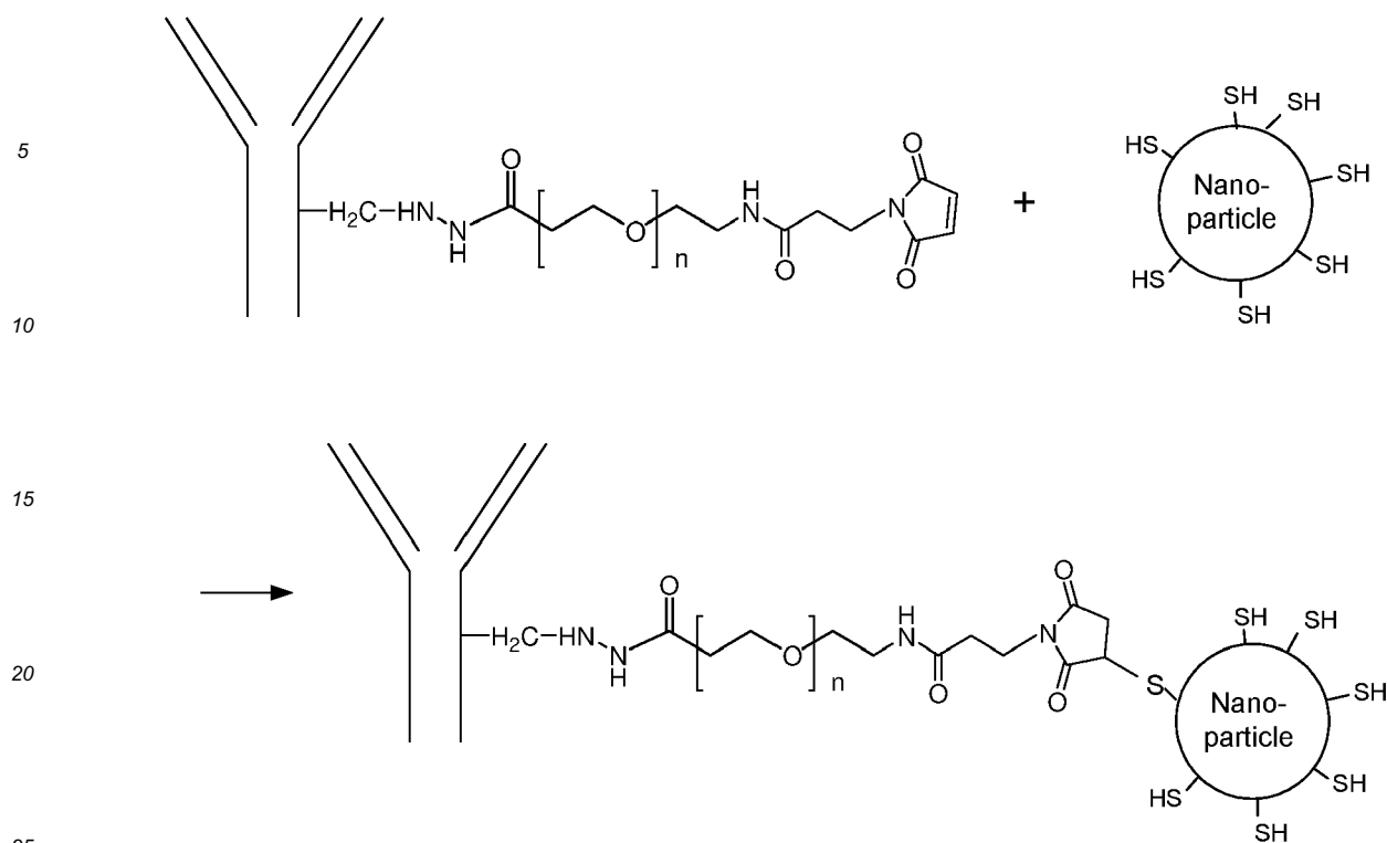
Scheme 23
