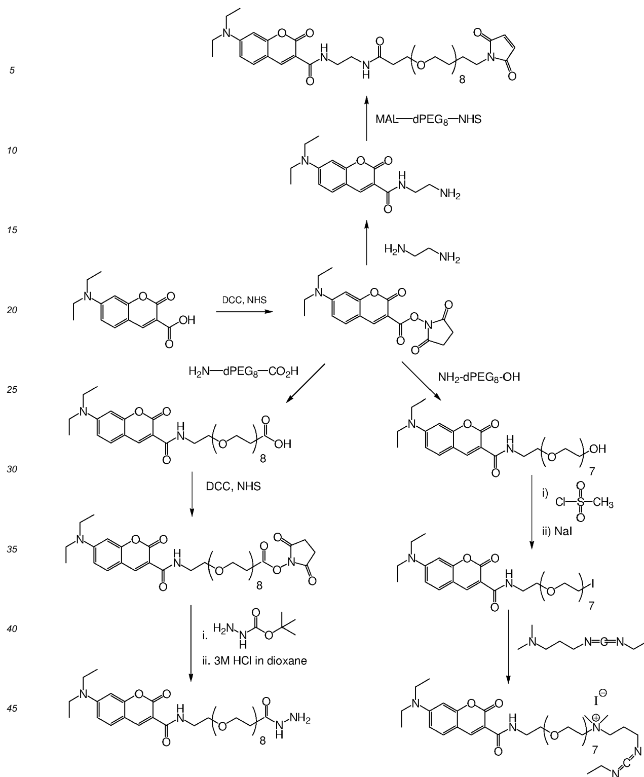
Scheme 11
