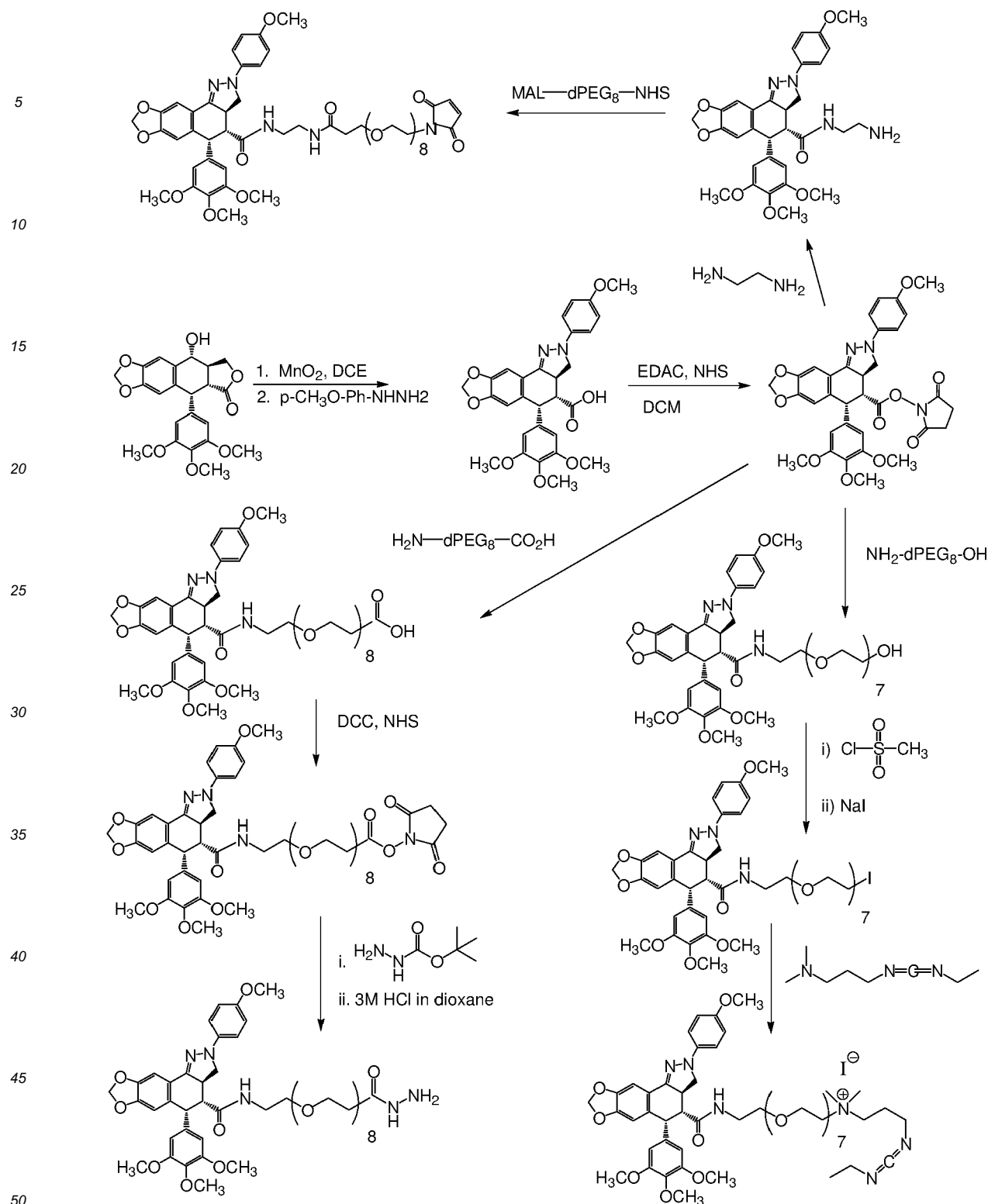
Scheme 12
