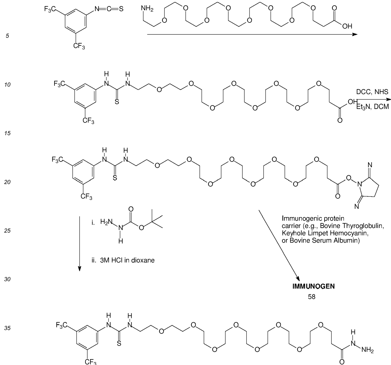
Scheme 7
