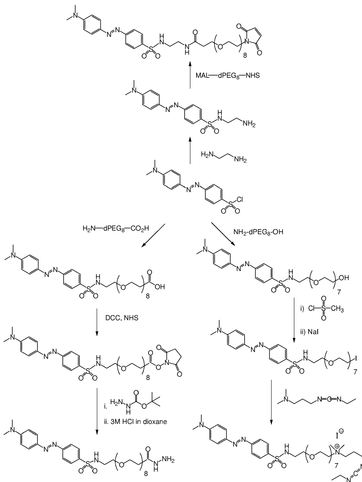
Scheme 15
