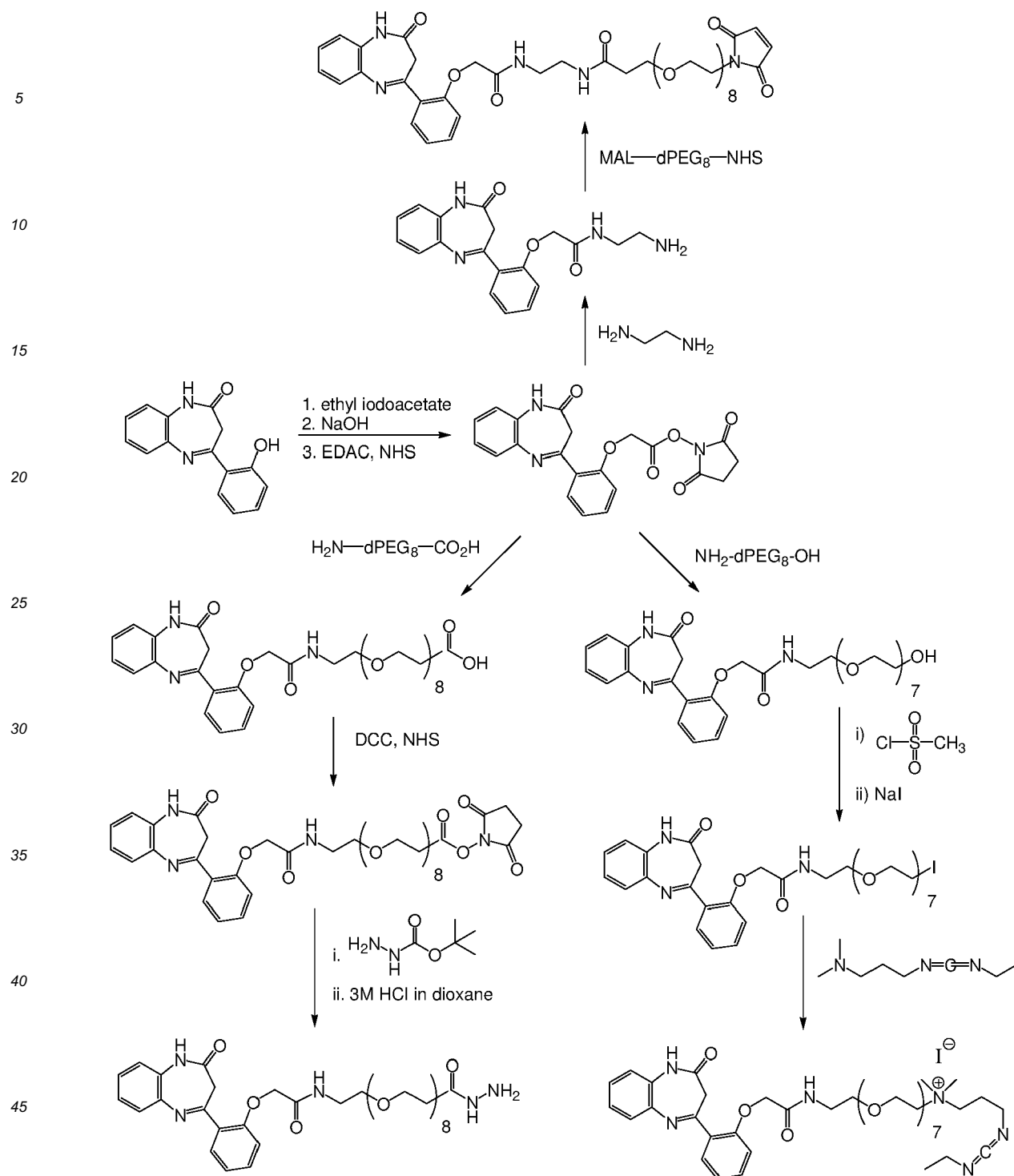
Scheme 16
