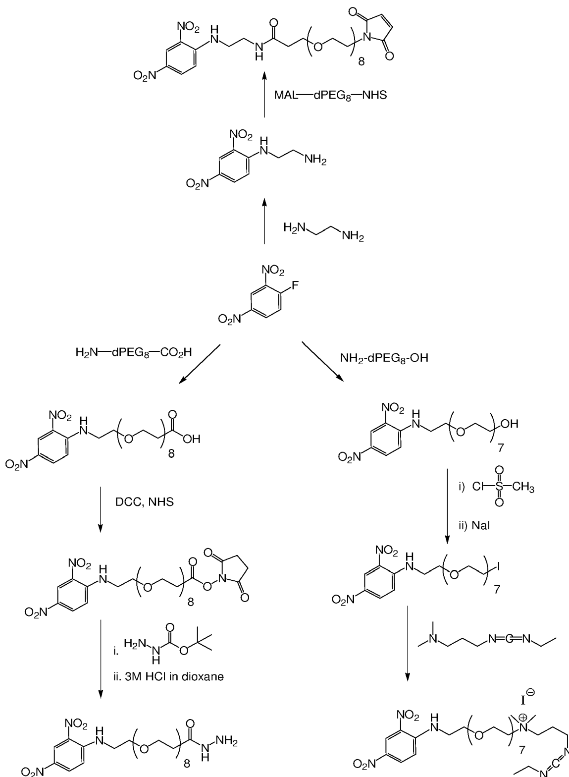
Scheme 2
