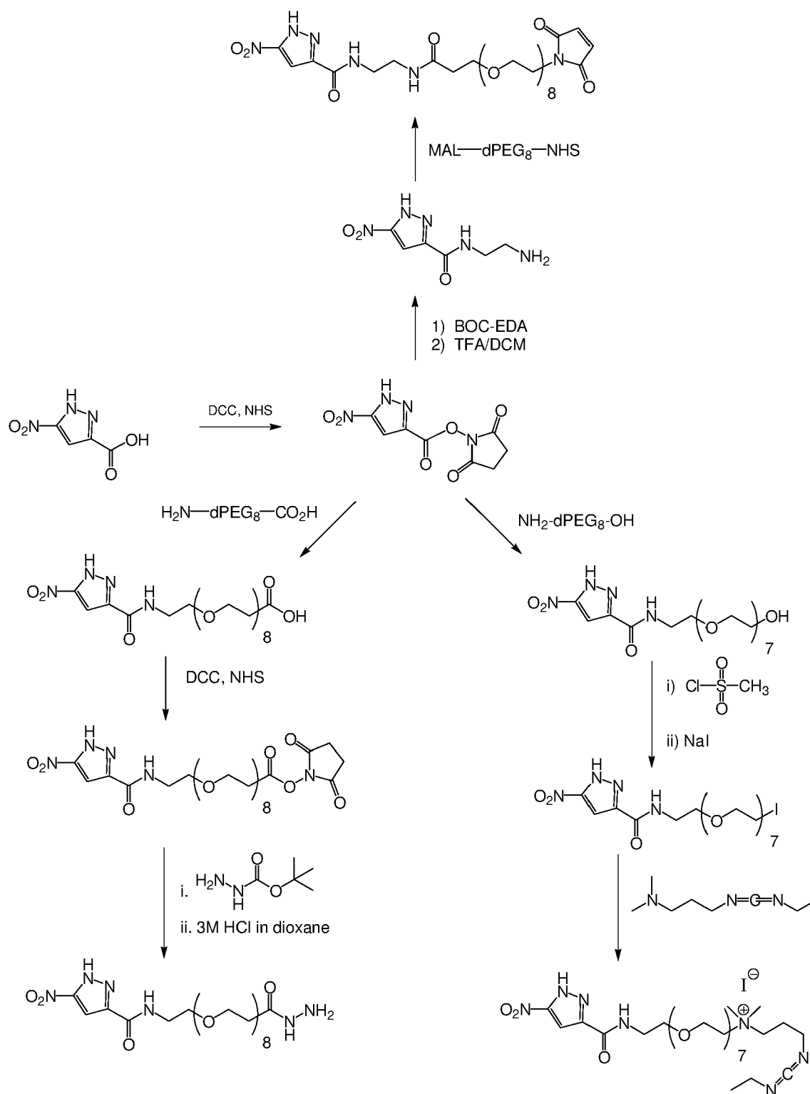
Scheme 1
