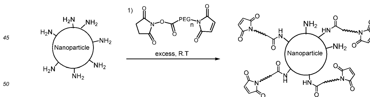
Scheme 19
