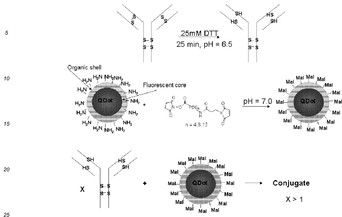
Scheme 24
