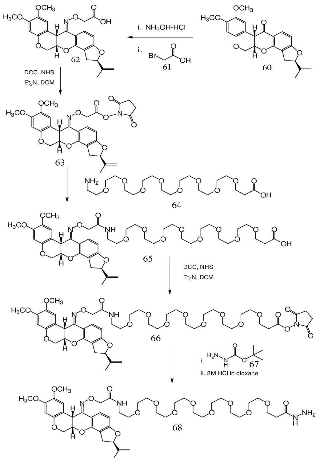
Scheme 8
