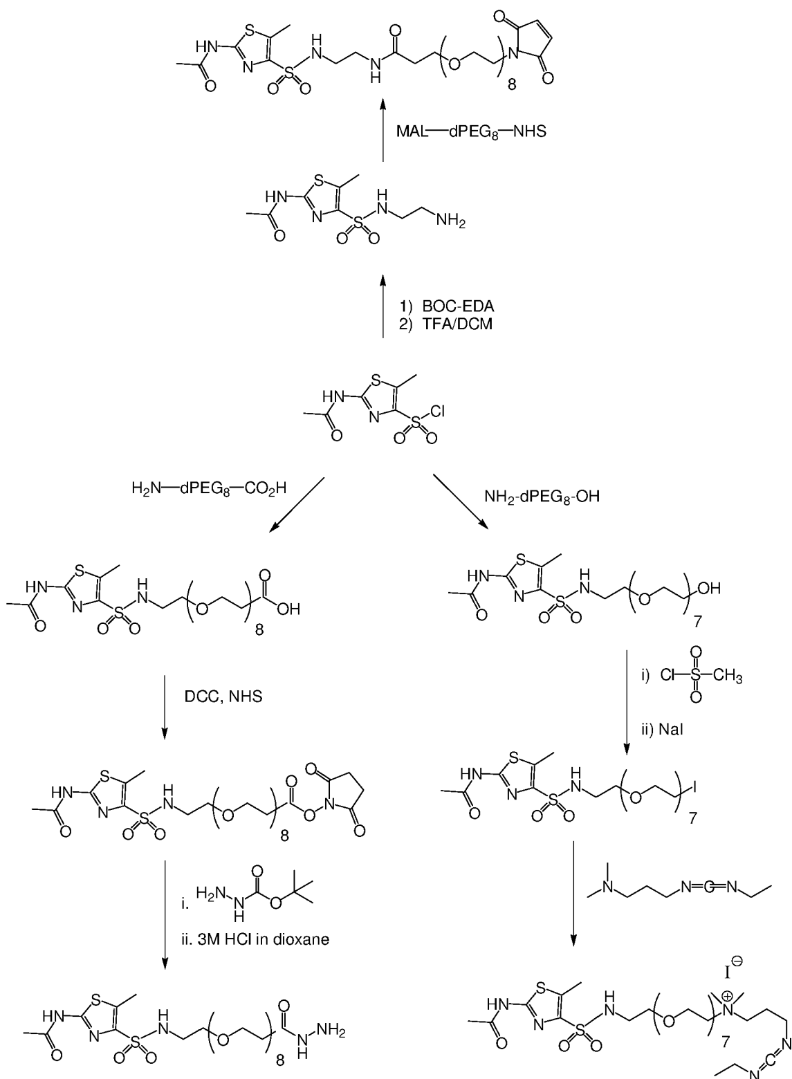
Scheme 10
