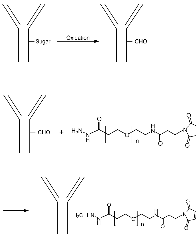
Scheme 22
