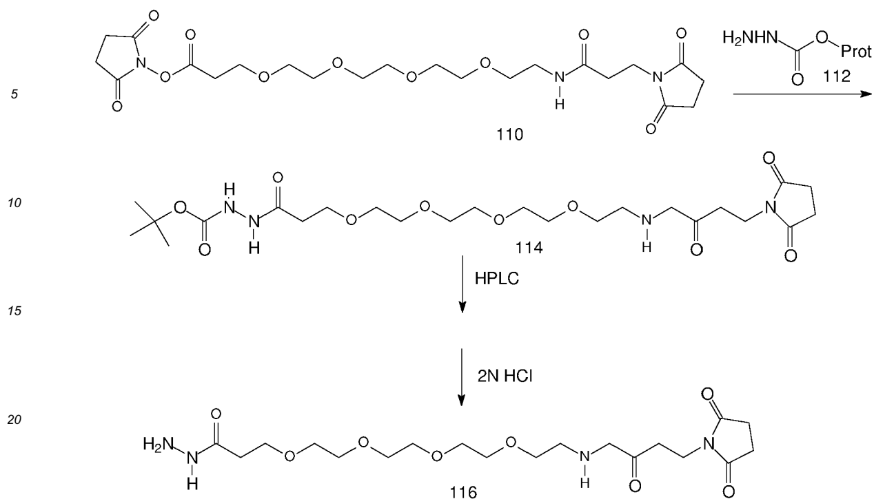
Scheme 18
