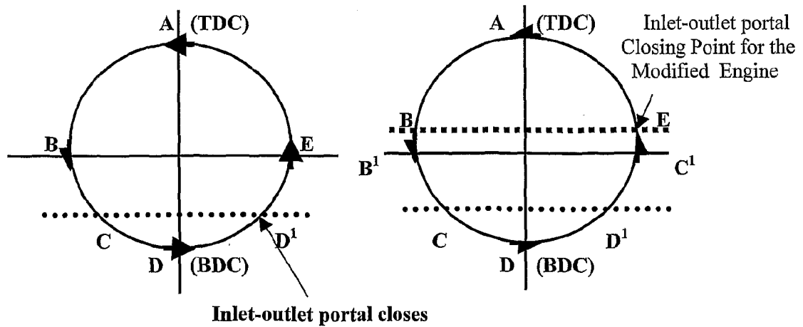
Schematic of angular rotation of the crank shafts (b) Conventional Engine (c) Modified Engine
