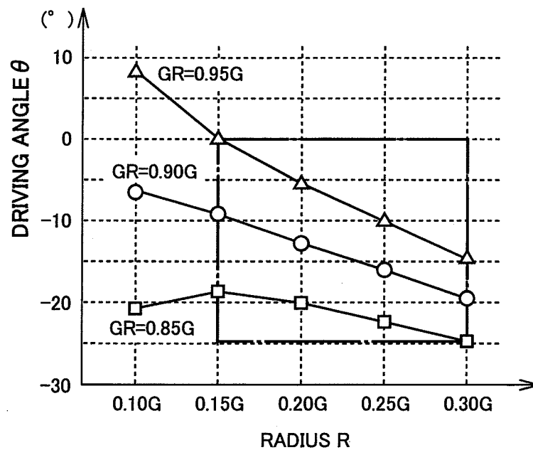
FIG. 3(b) GRAPH
