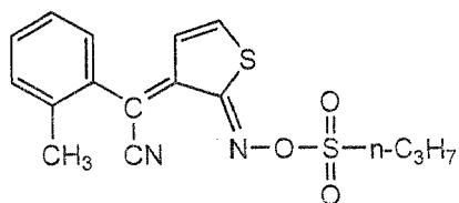
C2:IRGACURE PAG 108 (produced by Ciba Speciality Chemicals Co., Ltd.)
