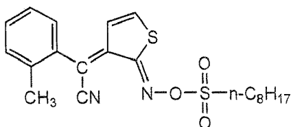
C3:CGI 1380 (produced by Ciba Speciality Chemicals Co., Ltd.)
