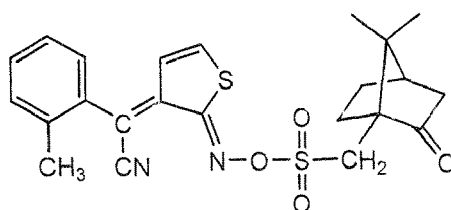
C4:IRGACURE PAG 121 (produced by Ciba Speciality Chemicals Co., Ltd.)
