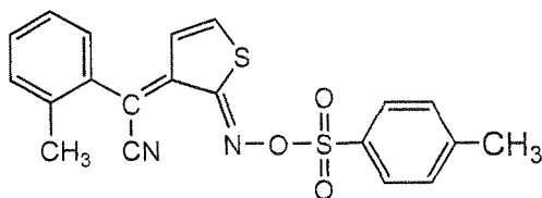
C5:CGI 725 (produced by Ciba Speciality Chemicals Co., Ltd.)
