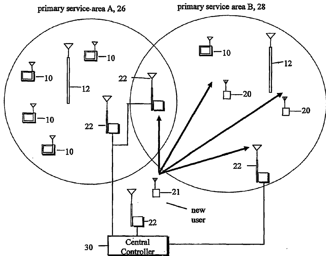
FIG. 2 New user's interference to primary users in service area B is estimated by signal strength measured by secondary users located in service area B.
