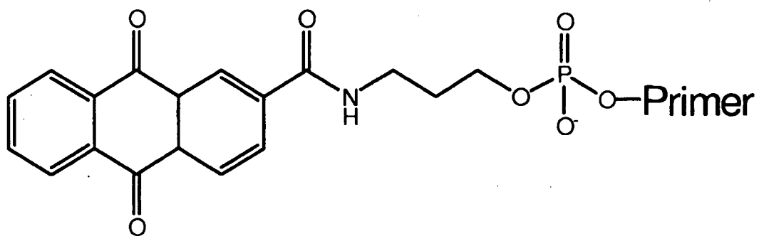
Anthraquinone (AQ)
