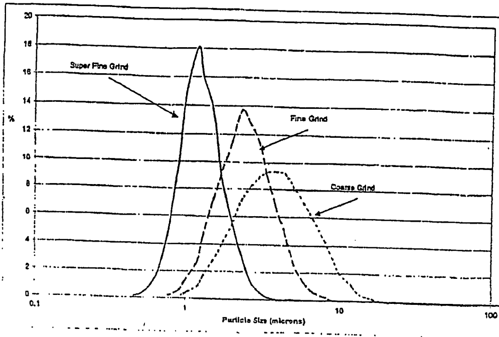
Figure 13 Particle size distributions for NbH particles.
