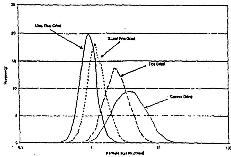
Figure 14 Particle size distributions for NbH powders.
