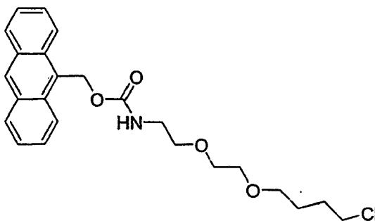
a compound of formula XXV
