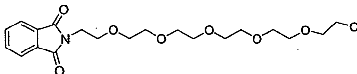
a compound of formula XXVIII
