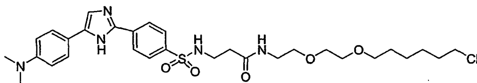
a compound of formula XVI
