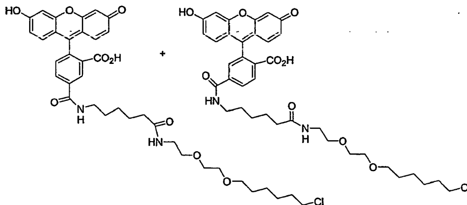
a compound of formula XXIII
