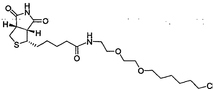
a compound of formula VII
