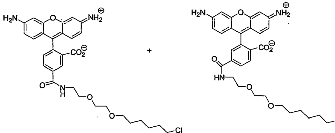
a compound of formula X
