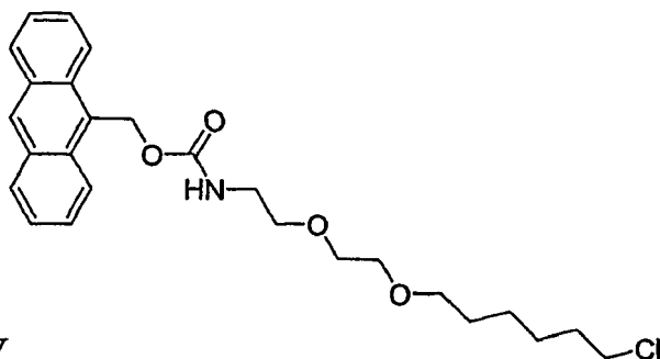
a compound of formula IV
