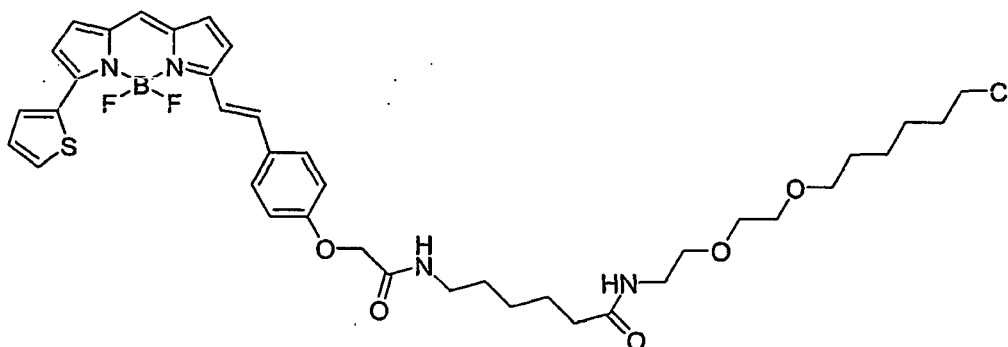
a compound of formula XIII
