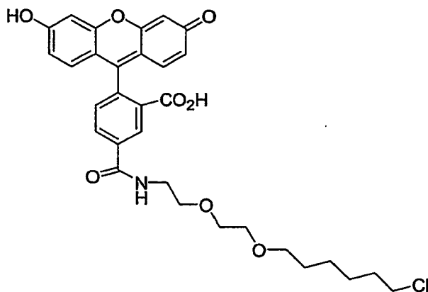
a compound of formula VI
