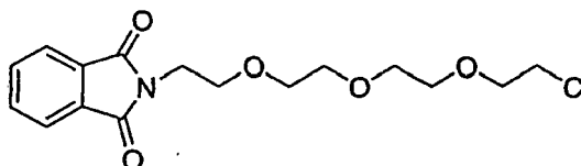
a compound of formula XXVI
