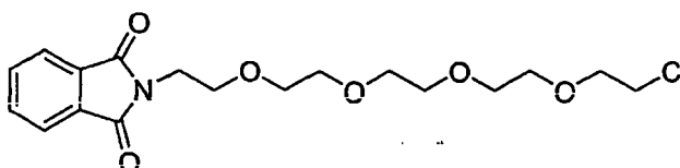
a compound of formula XXVII
