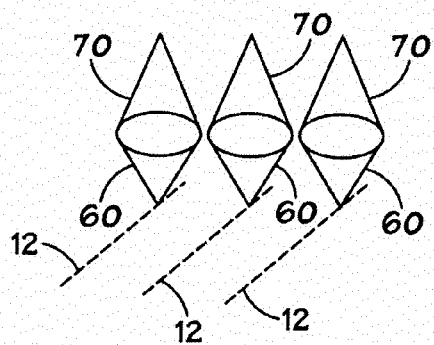
FIG. 4 ( MULTIPLE PICKUPS )
