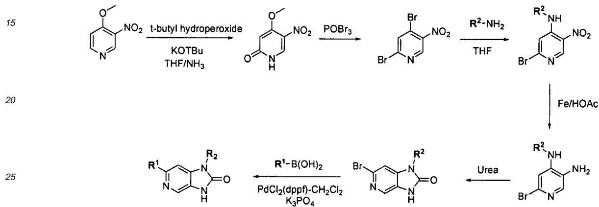
Scheme 4:
