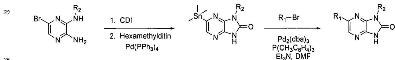
Scheme 12:
