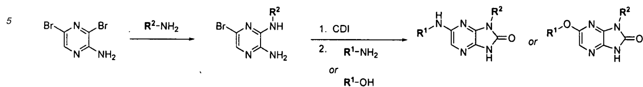
Scheme 4:
